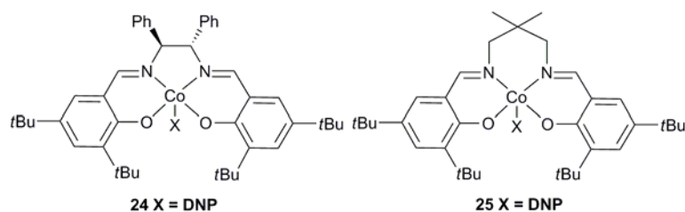
Figure 15. Cobalt salen complexes.
