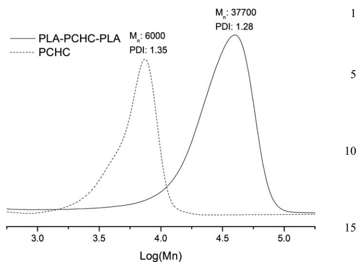
Fig. 3 Expanded overlaid GPC traces of PCHC and PLA-PCHC-PLA (entry 5, Table 1) using THF as an eluent.
