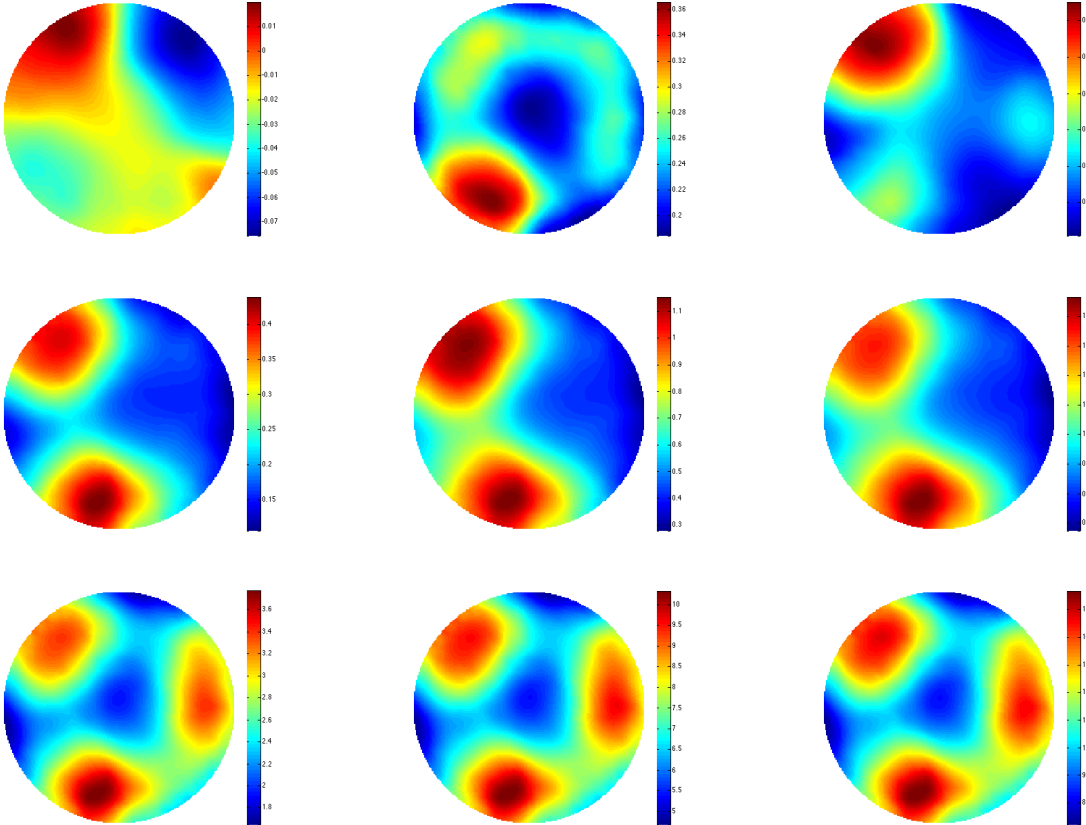
Figure 3: Reconstructed images for, by row, one, two and three inclusions of, by column, small, medium and large inclusions in a free space background. The conductivity of the inclusion is, by column, 1.52S/m, 4.06S/m and 5.94S/m respectively.
