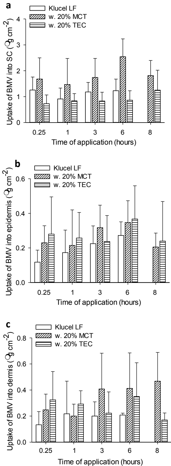
Supplementary Figure S2. Penetration profiles of BMV into the (a) SC, (b) epidermis and (c) dermis after topical application of Klucel FFS with and without TEC and MCT, plasticizer and lipid, respectively (mean \pm standard deviation; n=4).
