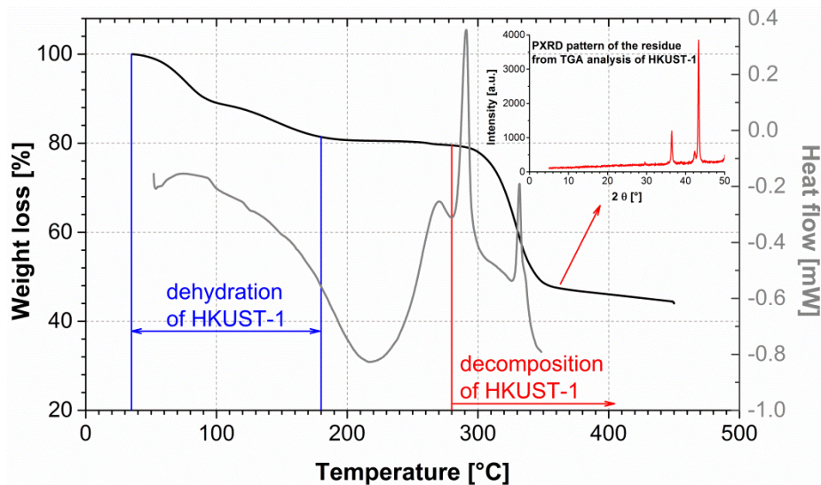
Fig. 4. TGA (under nitrogen) and DSC analysis of HKUST-1 framework synthesised at 100°C and 24 hours under static hydrothermal conditions. Inset: PXRD pattern of the residual material after TGA.
