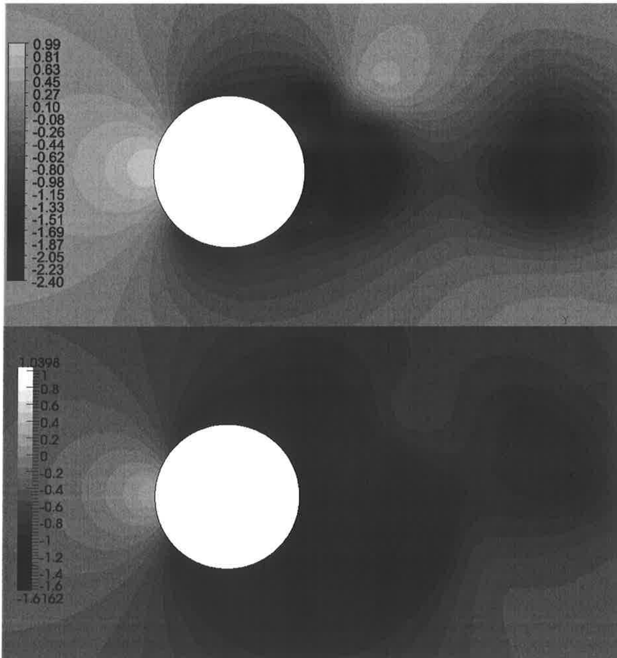
Fig. 9, Contour plots of pressure coefficient for Re = 10^4 ; Top: CFX, Bottom: OpenFOAM
