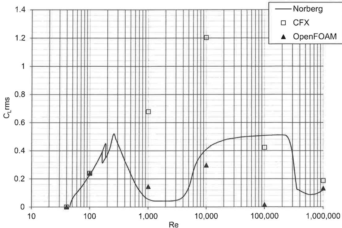
Fig. 7, Graph of rms value of lift coefficient with Reynolds number. Published experimental data: Norberg [13]
