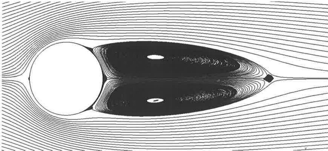
Fig. 3, Streamline and stagnation point images at Re = 40 after 150 non-dimensional seconds, Top: OpenFOAM, Bottom: CFX
