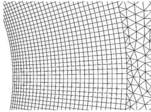
Fig. 2, Images of a typical mesh (Re=1000 shown); Top: Image showing near and far field meshes from the cylinder, Bottom: Detail of inflated hexahedral mesh at the cylinder boundary
