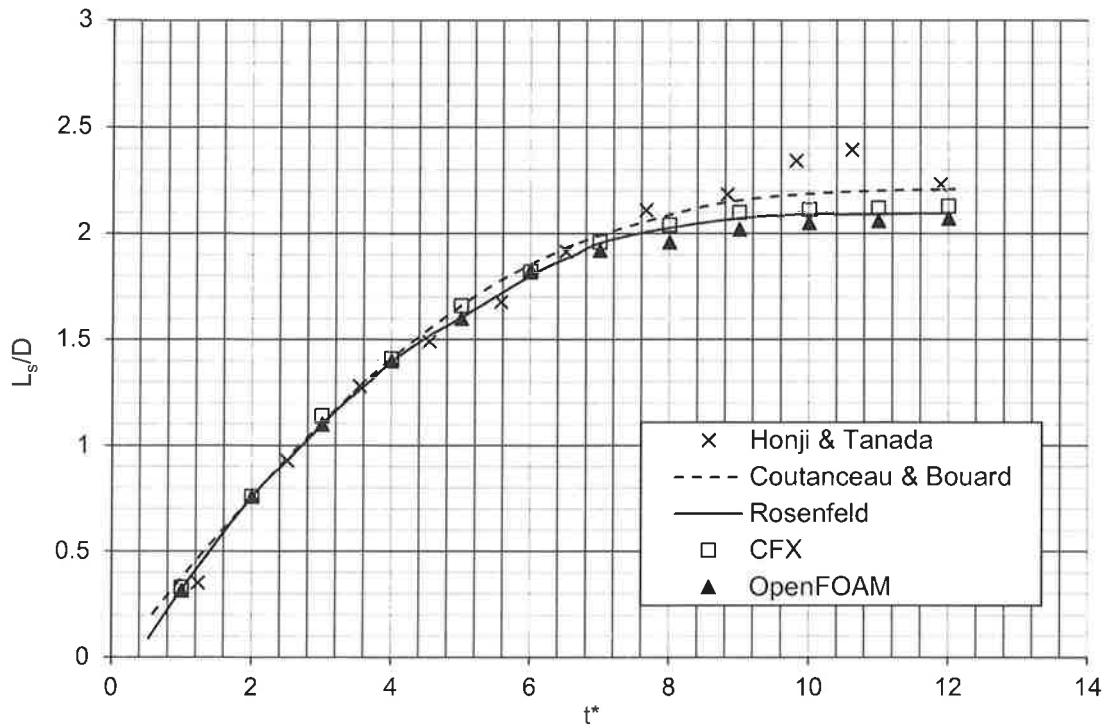
Fig. 4, Development of vortex length with respect to non-dimensional time. Experimental: Honji & Tanada [9]; Coutanceau & Bouard [4]; Numerical: Rosenfeld [10].
