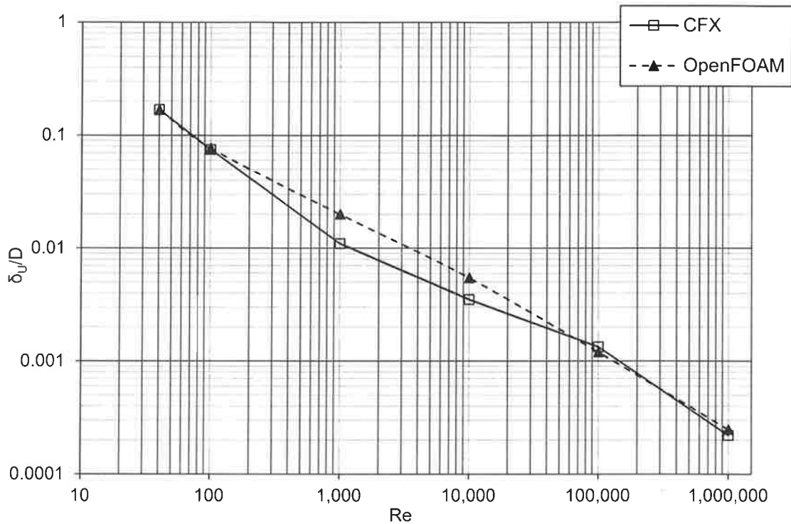
Fig. 10 Graph of non-dimensional boundary layer thickness versus Reynolds number.
