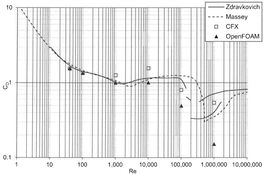
Fig. 5, Drag coefficient versus Reynolds number; correlation between experimental and numerical results. Published values for smooth cylinder: Zdravkovich [11] and Massey [12].
