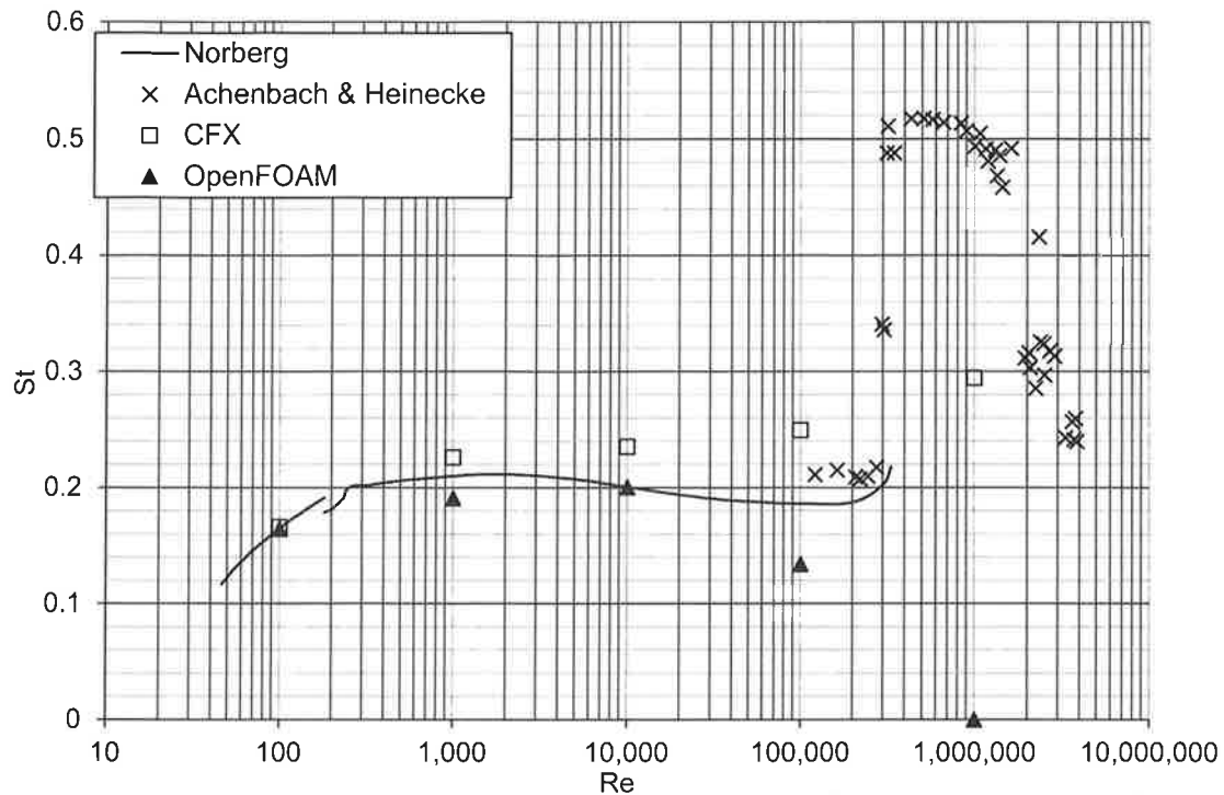
Fig. 8. Graph of Strouhal number with Reynolds number. Experimental data: Norberg [13]; Achenbach & Heinecke [14]
