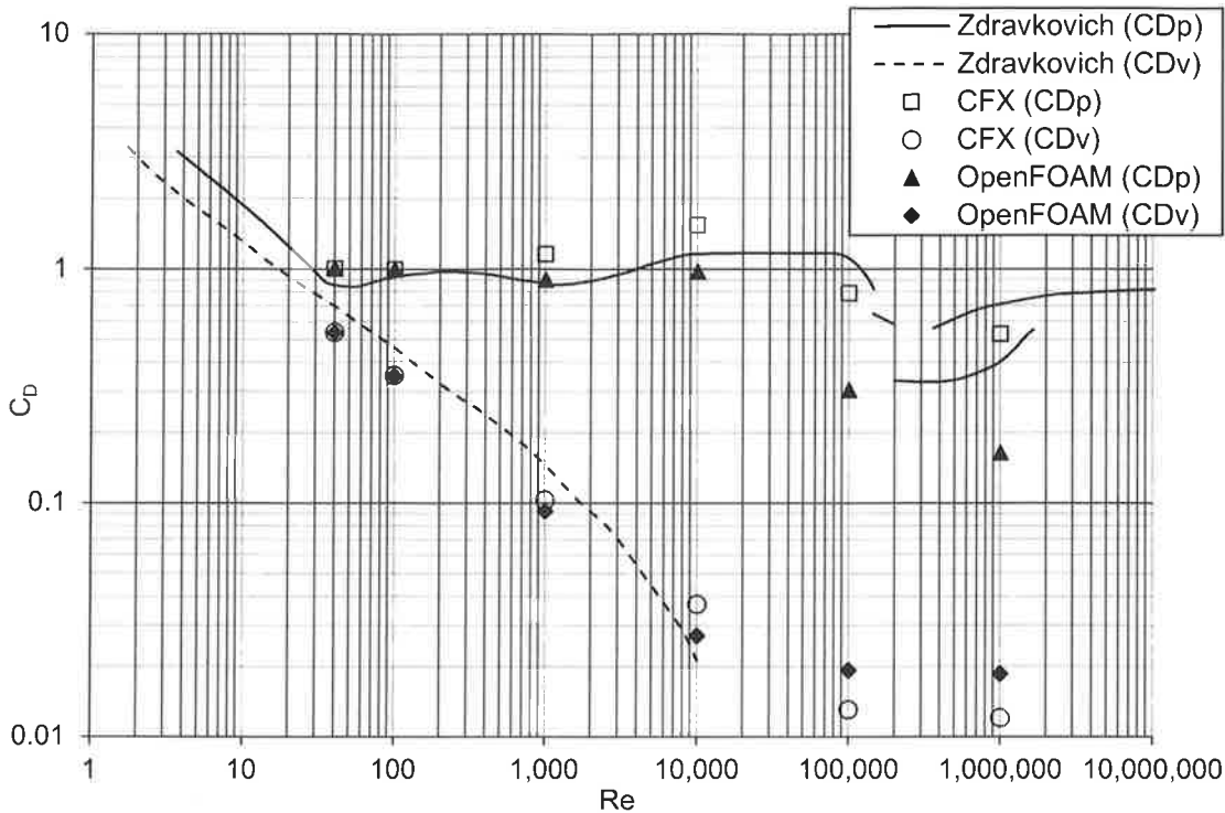
Fig. 6, Pressure and viscous components of drag coefficient versus Reynolds number. Published values for smooth cylinder: Zdravkovich [11].
