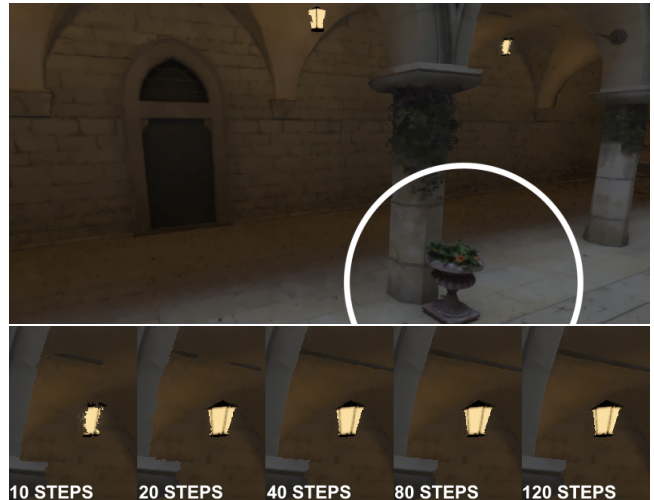
Figure 5: Top: Sample frame from our ray-casting method with 120 per-pixel steps in the foveal region (within circle) and 10 per-pixel steps in the peripheral region (outwith circle). Bottom: Close-up of right lamp showing artefacts across different quality levels.
