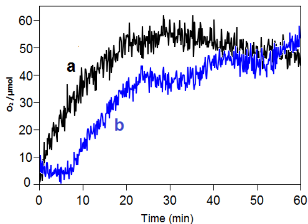
Fig.3 Visible light photocatalysed water oxidations showing O 2 yield with time using 5mWcm -2 blue light with (a) SiO 2 support containing Ru(bpy) 3 2+ and DCPIP with cobalt complex post absorbed; (b) repeat reaction using recovered, washed and degassed SiO 2 support with its incorporated reagents.
