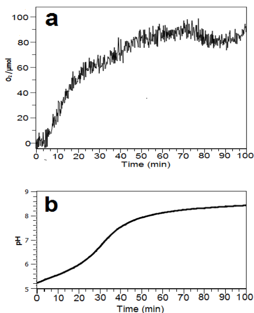
Fig. 2 (a) Visible light photocatalysed water oxidations showing O 2 yield with time using 5mWcm -2 blue light using 20mg of prepared Co(OH)(NH 3 ) complex as homogeneous catalyst; (b) change in pH of the reaction mixture with time.
