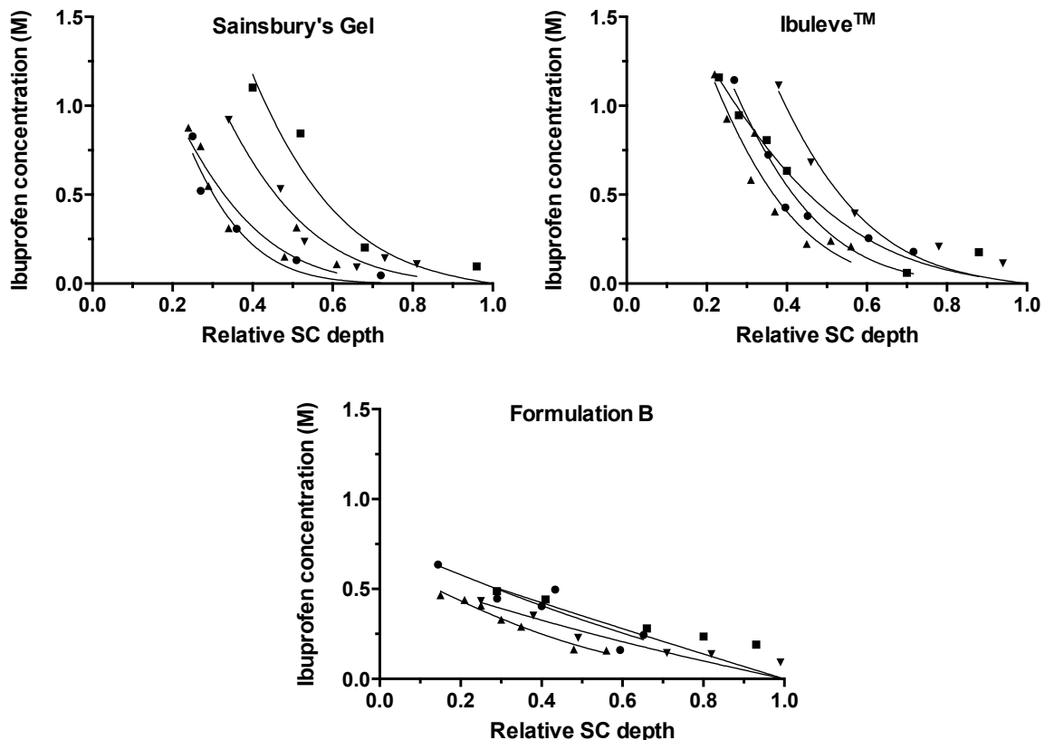
Figure 4: Concentration profiles of ibuprofen across human SC in vivo ( n = 4 ) following topical application of Sainsbury's Gel, Ibuleve™ and TOCN gel formulation B. The data are presented as a function of relative depth into the SC (where 0 represents the SC surface, and 1 indicates the interface between the SC and the underlying, viable skin layers).
