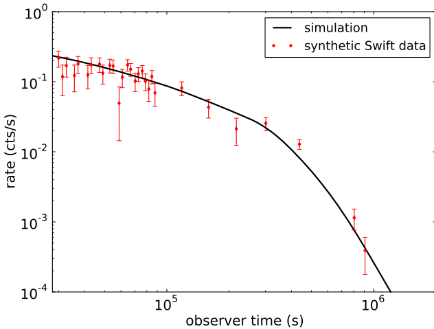
FIG. 8.— Synthetic Swift data generated from simulation light curve for an on-axis observer and p = 2.5 . The simulation flux has been scaled to a count rate of 0.1 cts/s at 1 day observer time.
