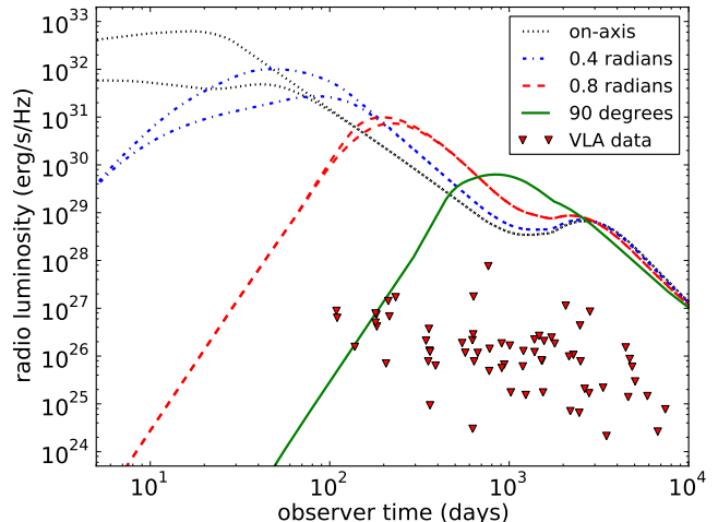
FIG. 12.— Analytically calculated light curves for different observer angles, with and without self-absorption. The observer frequency is set at 8.46 GHz. Self-absorption influences the light curves only until a few hundred days at most. At 8.46 GHz, the light curve for an observer at 90 degrees is the same with and without self-absorption enabled. The jet half opening angle is 11.5^\circ . The VLA late time radio limits for the local Ibc SNe are included as well.
