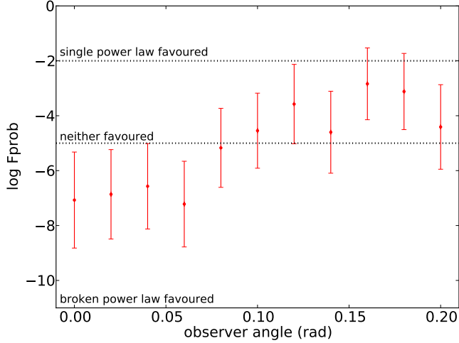
FIG. 10.— Results for F-test as function of observer angle. Note that a typical observer angle is 0.13.
