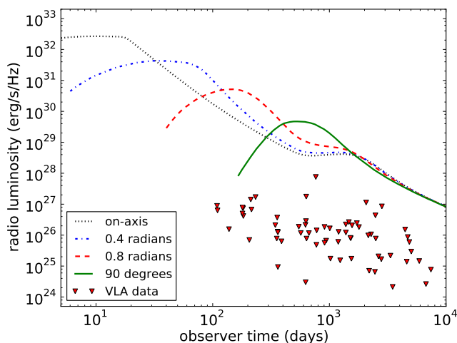
FIG. 11.— VLA late time radio limits ( 3\sigma ) for 66 local type Ibc of supernovae compared against simulation results. All supernova redshifts have been ignored (the largest redshift, that of SN 1991D, is \sim 0.04 ). The fluxes have been rescaled to luminosities. All VLA observations were done at 8.46 GHz, the afterglow light curve is calculated at the same frequency. As in the rest of this paper, the simulation jet half opening angle is 11.5^\circ .
