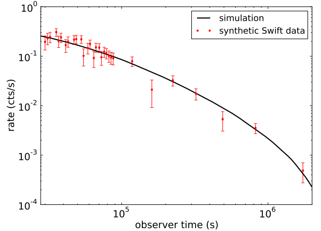
FIG. 9.— Synthetic Swift data generated from simulation light curve for an on-edge observer (i.e. at 0.2 rad) and p = 2.5 . The simulation flux has been scaled to a count rate of 0.1 cts/s at 1 day observer time.
