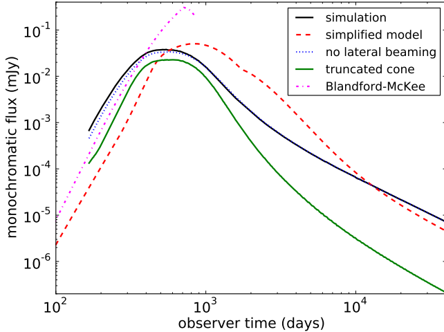
FIG. 7.— Light curves at 8.46 GHz for an observer at \theta_{obs} = 90^\circ . The simulation and simplified model curves are repeated from fig. 6. If we ignore the fluid velocity in the lateral direction for the purpose of the radiation calculation, we get the slightly lower curve labeled no lateral beaming . The emission is still well in excess of a light curve from a radiation calculation that takes the BM profile instead of the simulated fluid profile as input, labeled Blandford-McKee . Only by completely omitting the emission contribution from matter that has spread sideways out of the original jet opening angle, we get a flux level that is initially comparable to that of the exact BM solution and the simplified model. This is shown by the truncated cone curve.
