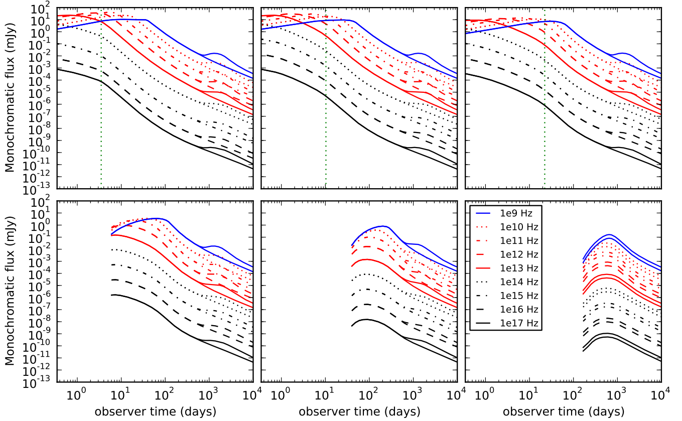
FIG. 1.— Simulated light curves for various observer angles and frequencies. On the top row we have small observer angles, 0.0, 0.1 and 0.2 radians from left to right. On the bottom row we have large observer angles, 0.4, 0.8 and 1.57 radians from left to right. Observer frequencies from 10^9 up to 10^{17} are plotted. For each frequency and angle a curve is plotted both with and without the contribution from the counterjet. The green vertical lines in the top plots indicate jet break time estimates using equation 4. The legend in the bottom right plot refers to all plots. Large observer angles are truncated at earlier time to show only observation times completely covered by the simulation.
