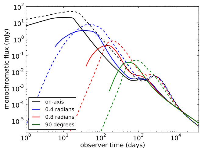
FIG. 6.— Direct comparison between simulation results (solid lines) and analytical model (dashed lines) for different opening angles, for radio frequency 8.46 GHz.
