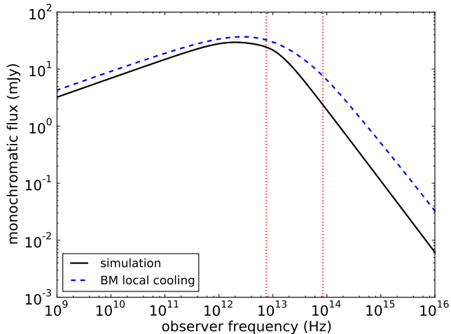
FIG. 4.— direct comparison between on-axis spectrum from simulation (solid curve) and BM solution with locally calculated cooling times (dashed curve), omitting self-absorption. The spectra are taken at 1 day in observer time, so well before the jet break. The leftmost vertical dotted line denotes the analytically calculated position of \nu_m , the rightmost that of \nu_c (calculated for the BM solution).
