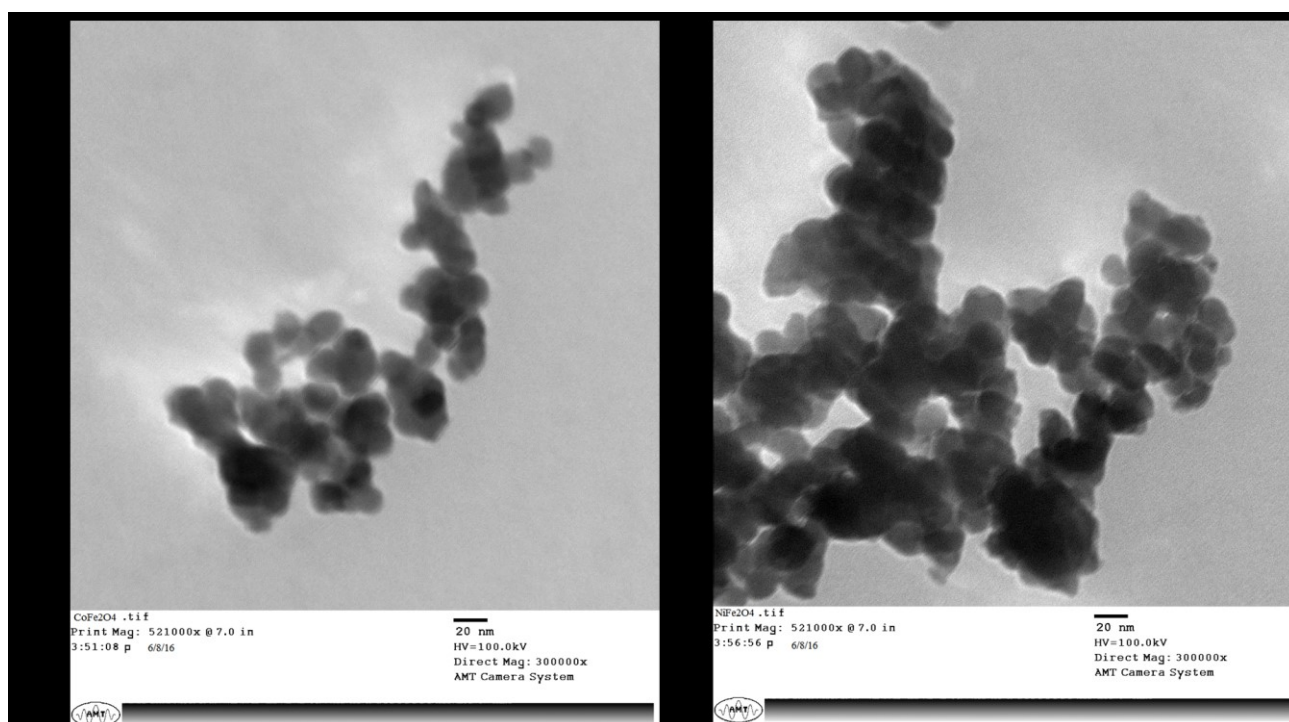
Figure 1. TEM images of (a) CoFe 2 O 4 and (b) NiFe 2 O 4 . Both nanoferrites show spherical nanostructures with an average size of 25nm.
