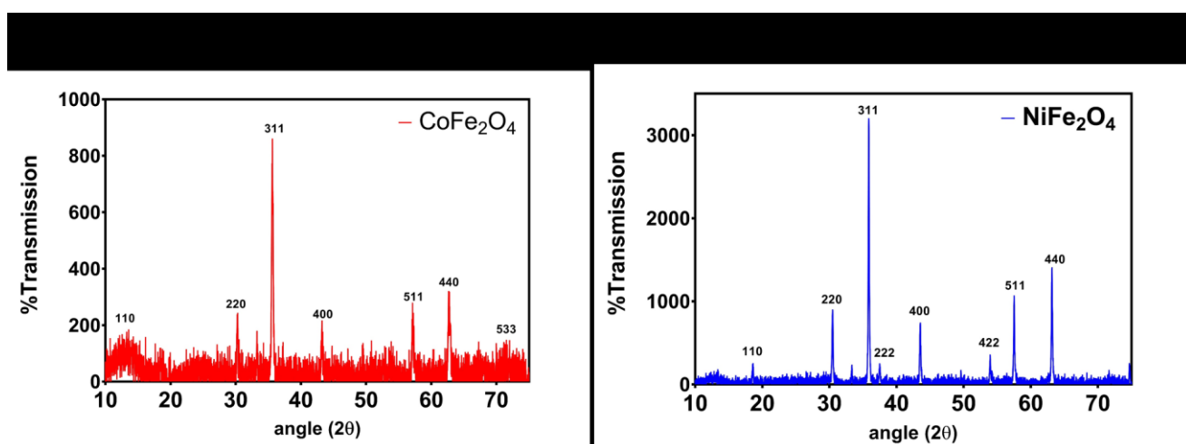
Figure 2. XRD images of (a) CoFe 2 O 4 and (b) NiFe 2 O 4 .
