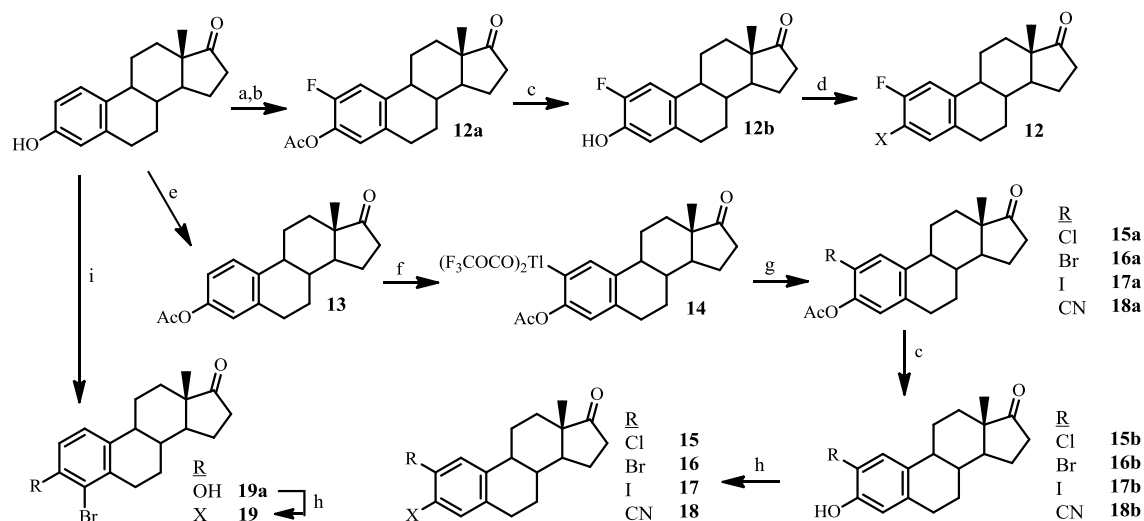
Scheme 4. Synthesis of 2- and 4-substituted derivatives of EMATE. a) N -fluoropyridinium triflate/1,2-trichloroethane, reflux, \text{N}_2 , 24 h; b) pyridine/acetic anhydride, reflux, 2 h; c) \text{K}_2\text{CO}_3/\text{MeOH} , reflux, 3 h; d) DBMP/DMF, \text{H}_2\text{NSO}_2\text{Cl} , 0^\circ\text{C} ; e) (\text{CH}_3\text{CO})_2\text{O}/\text{pyridine} , reflux, 2 h; f) \text{Ti}(\text{OCOCF}_3)_3/\text{CF}_3\text{COOH} , 0 - 5^\circ\text{C} , \text{N}_2 , 24 h; g) \text{CuX}/1,4\text{-dioxane} ( \text{X} = \text{Cl}, \text{Br}, \text{I}, \text{CN} ); h) \text{NaH}/\text{DMF} , \text{H}_2\text{NSO}_2\text{Cl} , 0^\circ\text{C} ; i) \text{Br}_2/\text{glacial acetic acid}/\text{powdered Fe} , r.t.. \text{X} = \text{OSO}_2\text{NH}_2
