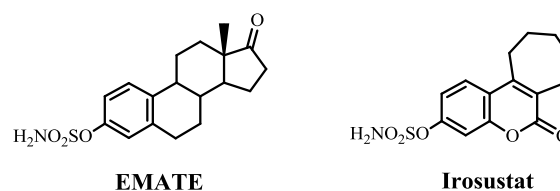
Figure 1. Structures of EMATE (estrone 3- O -sulfamate) and the non-steroidal STS inhibitor, Irosustat (STX64, BN83495).
