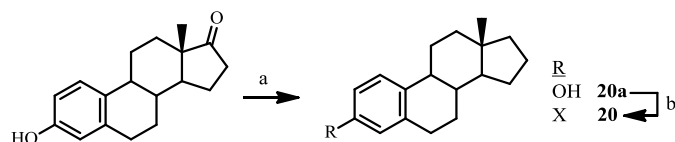
Scheme 5. Wolff-Kishner reduction of estrone and synthesis of sulfamate 20 . a) \text{NH}_2\text{NH}_2 \cdot \text{H}_2\text{O} , \text{KOH}/\text{diethylene glycol} , reflux; b) \text{NaH}/\text{DMF} , \text{H}_2\text{NSO}_2\text{Cl} , 0^\circ\text{C} . \text{X} = \text{OSO}_2\text{NH}_2
