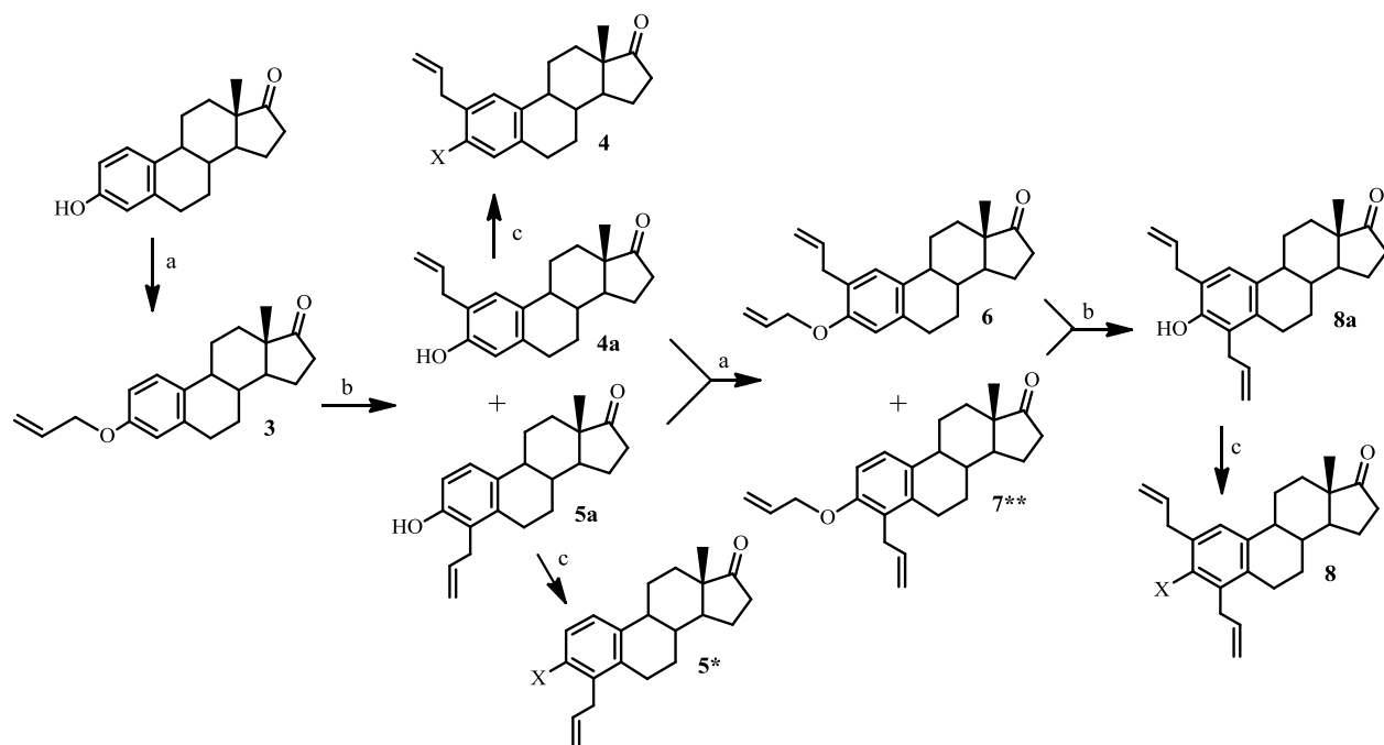
Scheme 2. Synthesis of 2-(2-propenyl)estrone 3- O -sulfamate ( 4 ), 4-(2-propenyl)estrone 3- O -sulfamate ( 5 ) and 2,4-di-(2-propenyl)estrone 3- O -sulfamate ( 8 ) via various intermediates ( 3 ), ( 4a ), ( 5a ), ( 6 ), ( 7 ) and ( 8a ). a) NaH/DMF, 3-bromoprop-1-ene, 80 °C, 2h; b) N,N -diethylaniline, N 2 , reflux, 6 h; c) NaH/DMF, H 2 NSO 2 Cl, 0 °C. X = OSO 2 NH 2 * contains ca. 25% of 4a as shown by 1 H NMR; ** impure, contains 6 .
