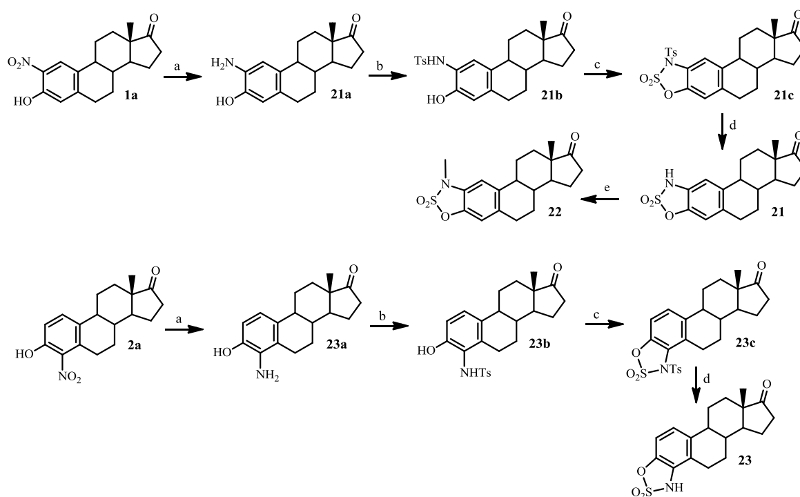
Scheme 6. Synthesis of 'cyclic' derivatives of EMATE. a) \text{Pd}/\text{C}(10\%)/\text{CH}_2\text{Cl}_2 , \text{H}_2 (balloon), 20 h; b) anhydrous pyridine, 0^\circ\text{C} , \text{TsCl} ; c) \text{Et}_3\text{N}/\text{CH}_2\text{Cl}_2 , \text{SO}_2\text{Cl}_2/\text{CH}_2\text{Cl}_2 (0.5 M), -78^\circ\text{C} ; d) \text{MeCN}/\text{aqueous KF} , reflux, 3 h; e) \text{NaH}/\text{DMF} , \text{MeI} , 90^\circ\text{C} , 3 h.
