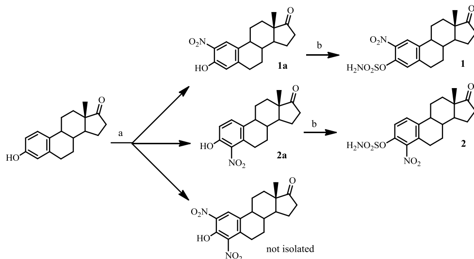
Scheme 1. Nitration of estrone to give predominately 2-nitroestrone ( 1a ) and 4-nitroestrone ( 2a ) which upon sulfamoylation gave their respective sulfamates ( 1 ) and ( 2 ). a) conc. HNO 3 /glacial acetic acid, 70-75°C to r.t.; b) NaH/DMF, H 2 NSO 2 Cl, 0 °C.
