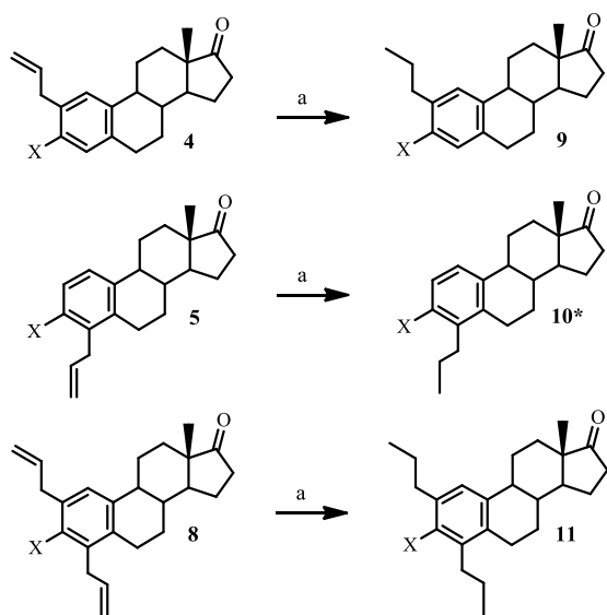
Scheme 3. Hydrogenation of (2-propenyl)estrone sulfamates ( 4 ), ( 5 ) and ( 8 ) to give respectively 2- n -propylestrone 3- O -sulfamate ( 9 ), 4- n -propylestrone 3- O -sulfamate ( 10 ) and 2,4-di- n -propylestrone 3- O -sulfamate ( 11 ). a) Pd-C(10%)/absolute EtOH, H 2 , 50 p.s.i. X = OSO 2 NH 2 * impure
