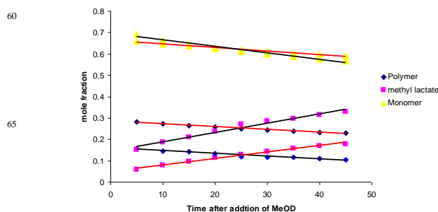
Fig. 1: Mole-fraction plots for the transesterification via depolymerisation of PLA and for the production of methyl lactate with Hf(1)(O i Pr) 2 – black line and Hf(2)(O i Pr) 2 red line.
