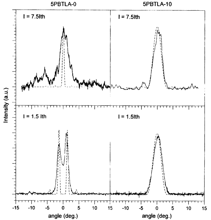
Fig. 5. Far-field intensity profiles measured under CW operation (solid line) and above threshold ( I = 7.5I_{th} ), from (a) 5PBTLA-0s and (b) 5PBTLA-10s. (No lenses were used; angle resolution: 0.05 deg.) Corresponding theoretical profiles (dashed line) obtained with the coupled mode theory are also presented for completeness.
