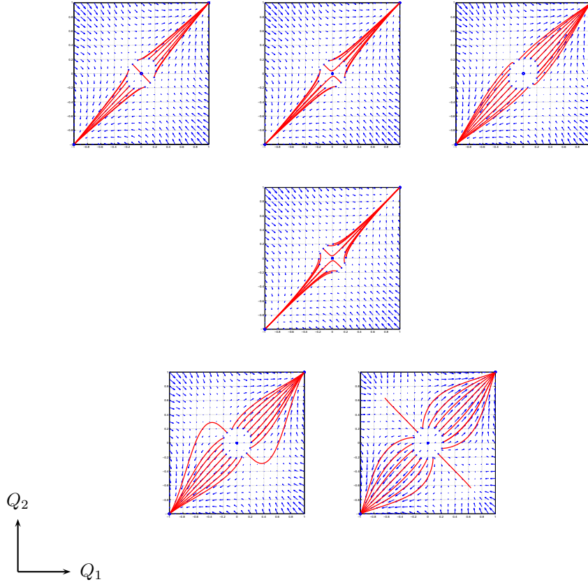
FIGURE 4. Example phase planes for the predisperal learning model (22). Parameter values are \mu = 0.4, \sigma = 0.2 throughout. In the top row, \epsilon = 0.25 , so that \lambda_2 < \lambda_1 < 0 and anti-symmetric steady states never appear for any \lambda > 0 , but they are unstable for all \lambda > 0 . In these simulations, \lambda = 0 and \lambda = 0.2 for illustration. In the middle row, \epsilon = 0.18 , so that \lambda_1 > 0 but \lambda_2 < 0 . In other words, anti-symmetric steady states do form for \lambda < \lambda_1 (in this illustration, \lambda = 0.1 < 0.156 \equiv \lambda_1 ), but they are never stable for any \lambda > 0 . In the bottom row, \epsilon = 0.1 . For these values of \epsilon and \sigma , \lambda_1 \equiv 0.625 , and \lambda_2 = 0.405 . Hence, with sufficiently little learning, dialects are formed. From left to right in this row, \lambda = 0.8, 0.5, 0.2 .
