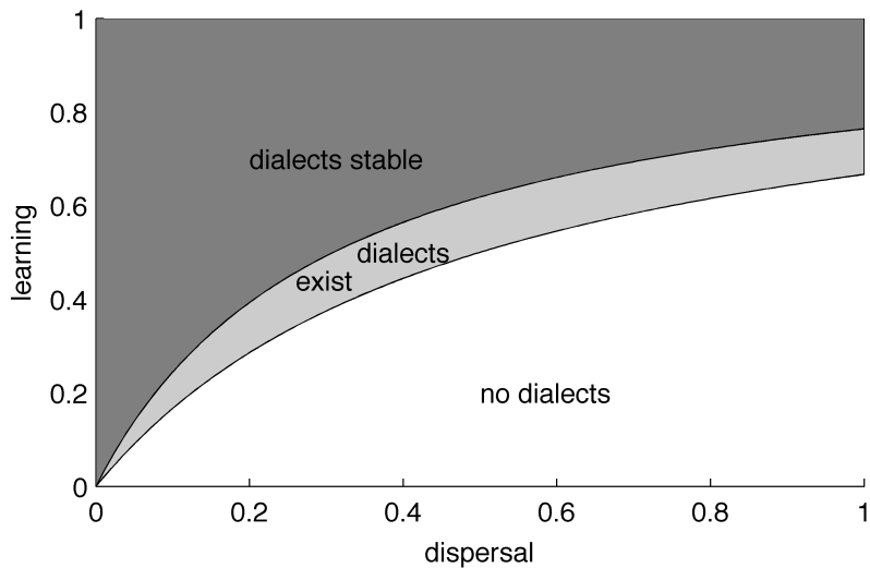
FIGURE 6. Bifurcation diagram of the nonlinear frequency-dependent learning model, indicating for which parameter values dialects exist or are indeed stable. The dark-gray area indicates the region of stable dialects for the choice z = 2 , see inequality (53).
