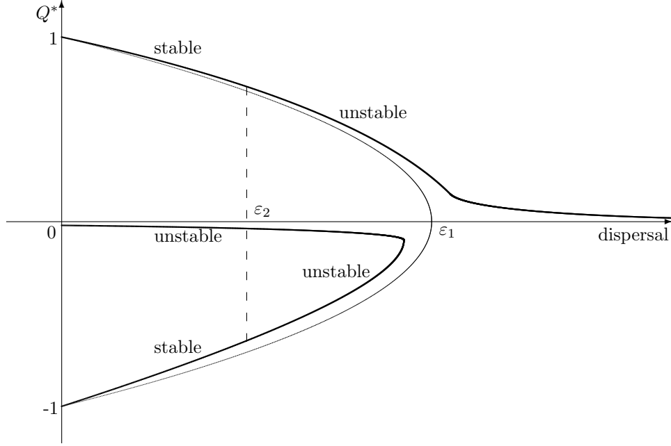
FIGURE 5. The bifurcation diagram for Model 3.
