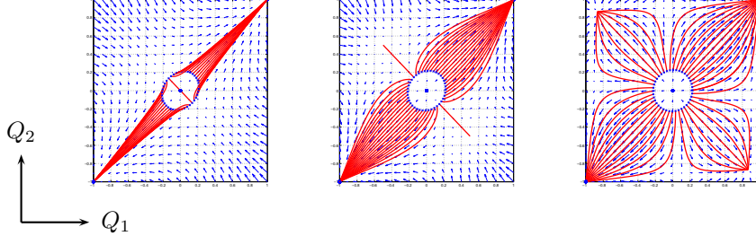
FIGURE 2. Example phase planes for system (8). Parameter values are \lambda = 0.4, \mu = 0.4, \sigma = 0.2 throughout, and \varepsilon = 0.25 (left), \varepsilon = 0.15 (middle) and \varepsilon = 0.05 (right). The critical \varepsilon -values at which bifurcations occur are \varepsilon_1 = 0.2 and \varepsilon \approx 0.14 . As \varepsilon decreases, the nontrivial dialect steady states bifurcate from the origin, are first unstable (middle plot), and then become stable (right plot). Arrows indicate direction and speed of change of the dynamical system. The red lines are example solutions with initial conditions chosen on a circle centered around the origin. These plots illustrate how far the nontrivial steady states extend away from the origin before they stabilise, and also give some indication of the basins of attraction of these dialect steady states.
