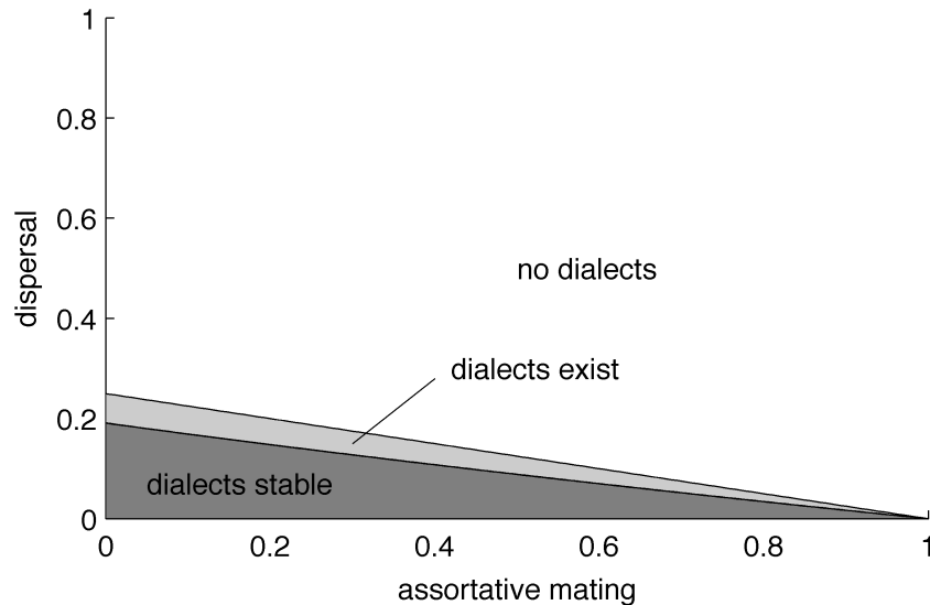
FIGURE 1. Bifurcation diagram for the post-dispersal learning model, indicating for which parameter values dialects exist or are indeed stable, summarised in inequalities (13) and (21).
