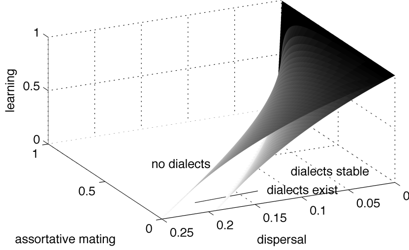
FIGURE 3. Bifurcation diagram for the pre-dispersal learning model, indication when dialect steady states exist or are indeed stable, summarised in inequalities (25) and (27).
