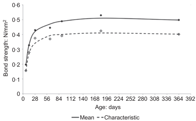
Figure 5. Bond strength data for a 12 part 40% sodium silicate solution to 60 parts sand/clay mortar with Ecoterre bricks
