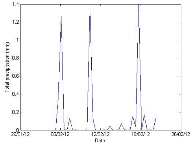
Fig. 5. Precipitation over the measured domain
