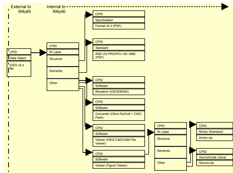
Figure 3. Graphical visualization of part of an RI Network for the IGES 5.3 file format 20 .
