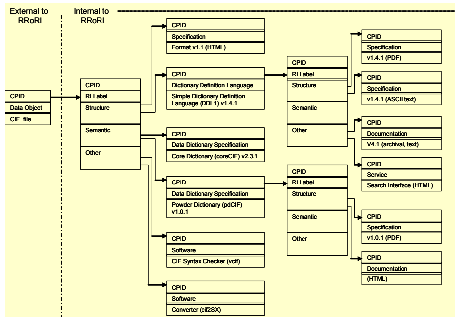
Figure 2. Graphical visualization of part of an RI Network for the CIF file format. 18
