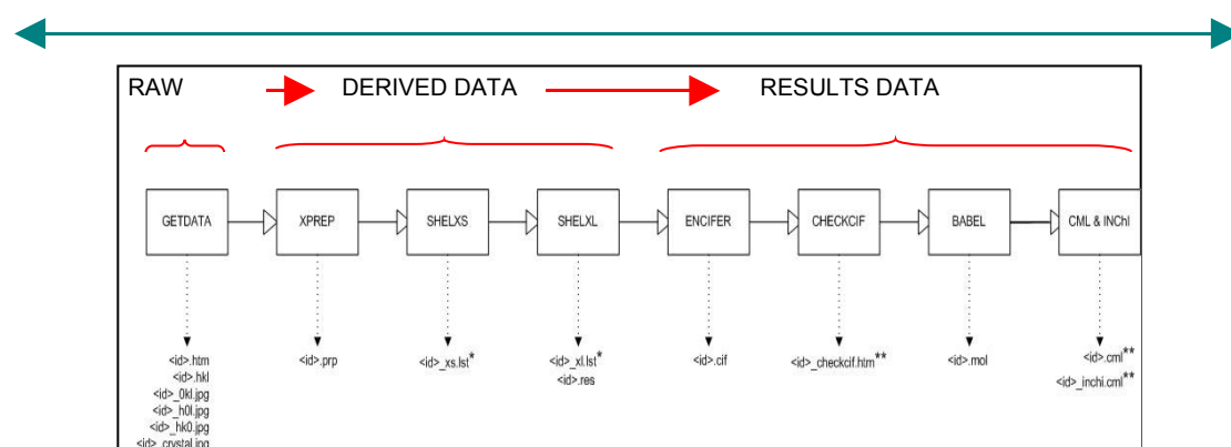
Figure 1. Workflow model of the EPSRC UK National Crystallographic Centre (NCS).
