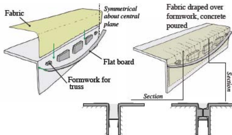
Figure 8: Pinch mould
