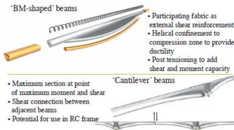
Figure 11: Future innovations for fabric-formed structures
