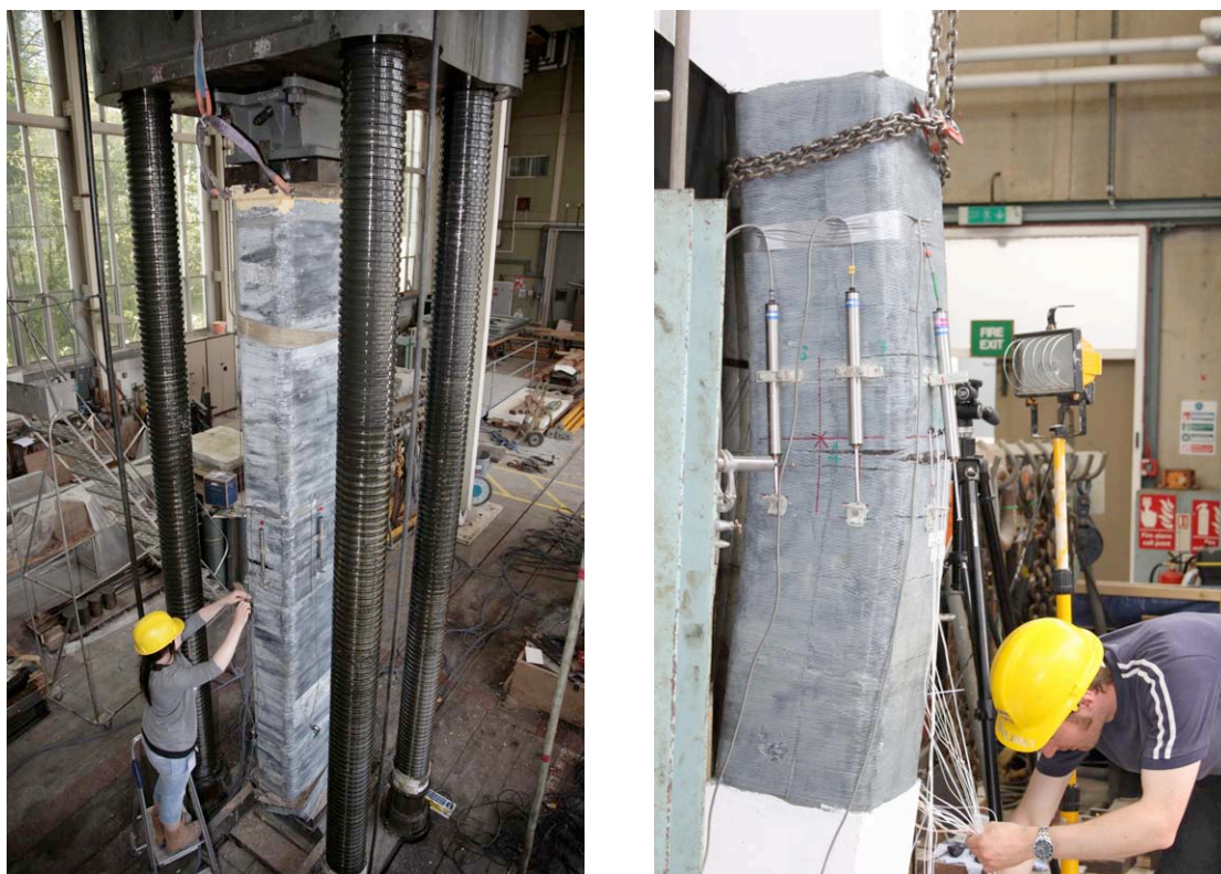
Figure 1: Large-scale FRP-wrapped column testing
