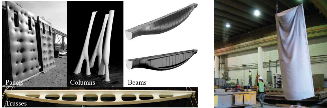
Figure 3: Fabric formed structures (after West [7]; Garbett [8])
