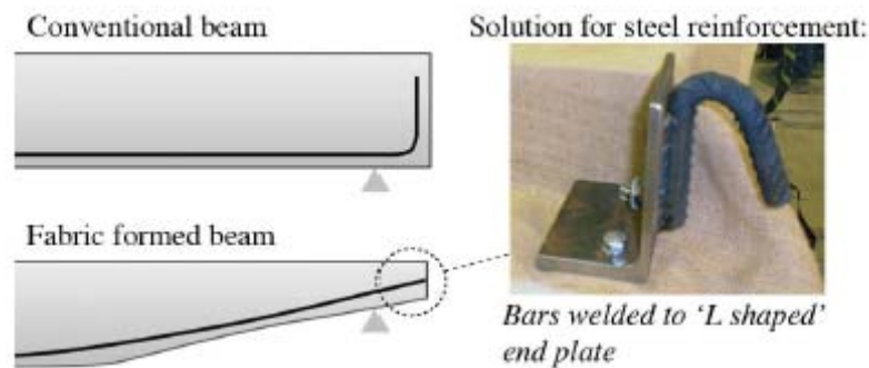
Figure 5: Present unsatisfactory anchorage connection
