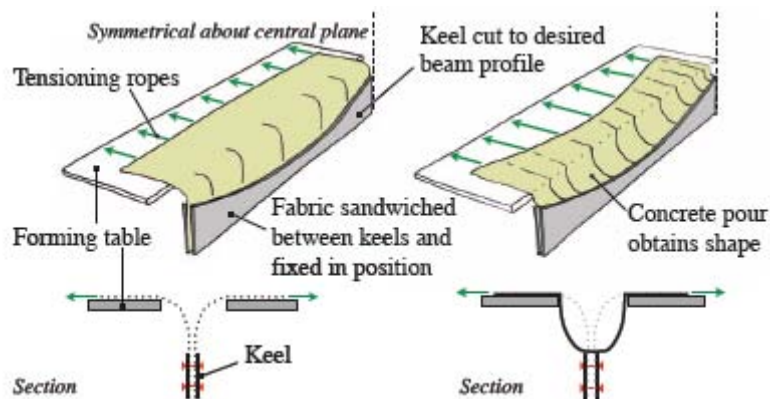
Figure 7: Keel mould
