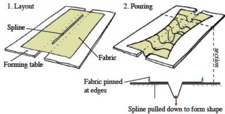
Figure 6: Spline method
