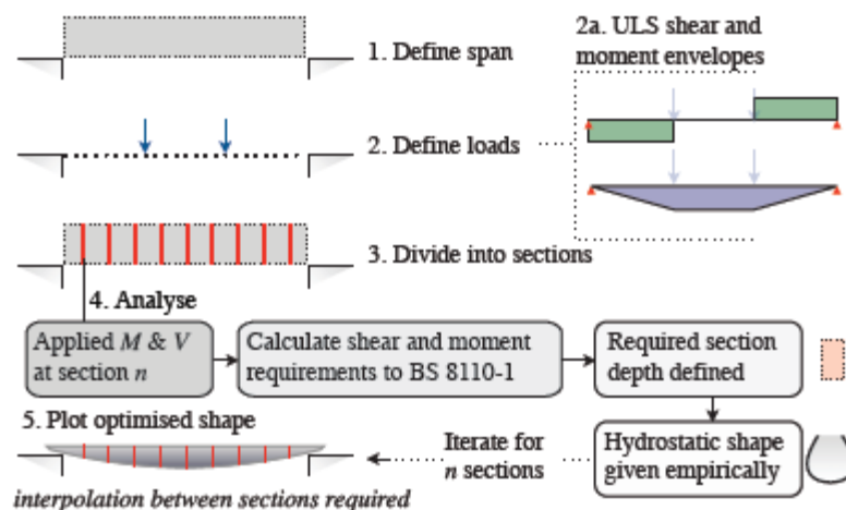
Figure 4: Sectional design method
