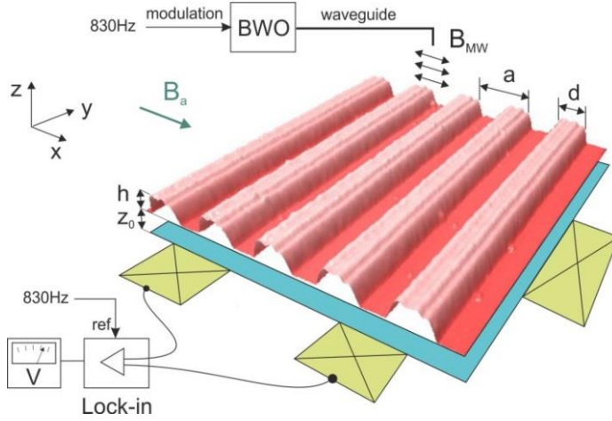
Fig. 1. Ferromagnetic finger gates fabricated on a GaAs/AlGaAs heterojunction. The fingers are magnetized by magnetic field B_a and irradiated by linearly polarized microwaves – magnetic field B_{MW} – supplied by a backward wave oscillator (BWO). Magnetic excitations are detected through the photovoltage they induce in the high mobility 2DEG.
