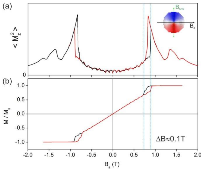
Fig. 4. Hysteretic effects associated with vortex core penetration in a Dy dot (a) ferromagnetic resonance calculated using OOMMF when the magnetic field is swept up/down; (b) simulated magnetization curve.
