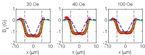
FIG. 4. (Color online) Experimental magnetic field profiles (circles) across mesoscopic \text{Sr}_2\text{RuO}_4 disks ( R=5\mu\text{m} ) captured after field-cooling from T > T_c to T=260\text{mK} in applied fields of 30, 40 and 100Oe. Two theoretical fits are shown. First, assuming a constant bulk critical current J_c = 7.75, 6.5 and 6.0 \times 10^4 \text{Acm}^{-2} respectively (dotted lines), and a second assuming edge supercurrents ( J_E = 1.55, 1.25 and 1.15 \times 10^6 \text{Acm}^{-2} respectively) flowing within d/2 of the edge of the disk and J_c = 0 (solid lines).
