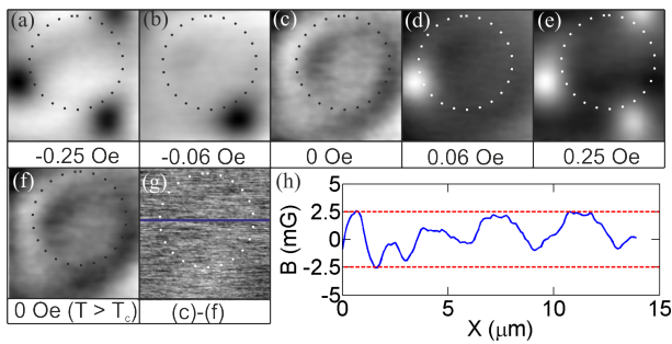
FIG. 2. (Color online) SHPM images ( 14\mu\text{m} \times 14\mu\text{m} ) of a mesoscopic \text{Sr}_2\text{RuO}_4 disk (dashed line - R=5\mu\text{m} ) after field-cooling in small fields spanning H_{\text{eff}} = 0 Oe. T=260\text{mK} . From left to right the image grayscales (G) are: 0.41, 0.45, 0.18, 0.42 and 0.44, 0.19, 0.07 G. The similarity of the images at H_{\text{eff}} = 0 , above and below T_c [(c) and (f)] indicates that any contrast in these images is entirely attributable to a gating artefact. The linescan (h) from the difference (g) [image (f) minus image (c)] places an upper limit of \pm 2.5\text{mG} on spontaneous fields due to chiral edge currents in these images.
