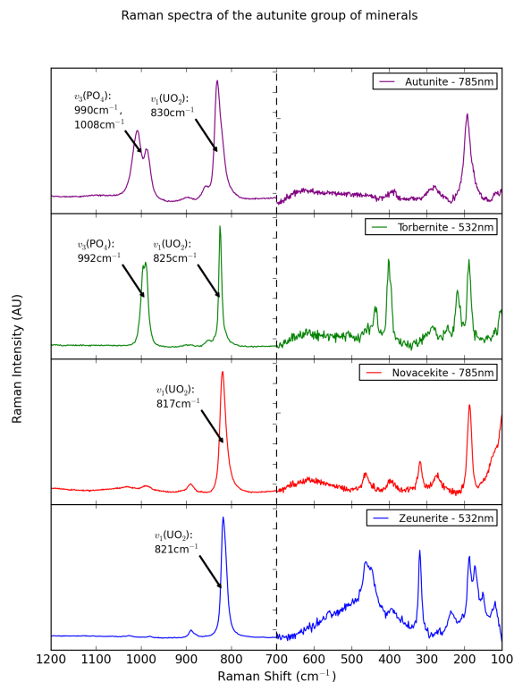
Fig. 2 Representative Raman spectra of autunite, torbernite, nováčekite and zeunerite mineral samples. The 100\text{--}700\text{cm}^{-1} region has been rescaled, to emphasise the bands in this region. The wavelengths displayed correspond to the optimum excitation for each mineral. The major peaks are annotated, while all bands are listed in Tables SI 1–4.
