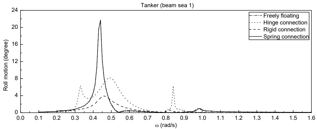
Figure 11. Roll responses in Beam Sea-1
