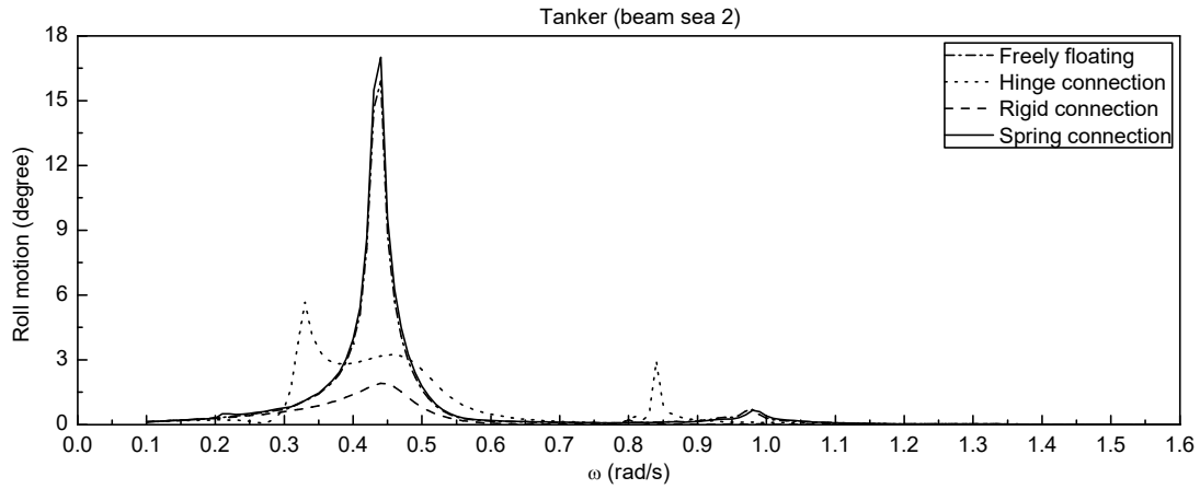
Figure 16. Roll responses in Beam Sea-2
