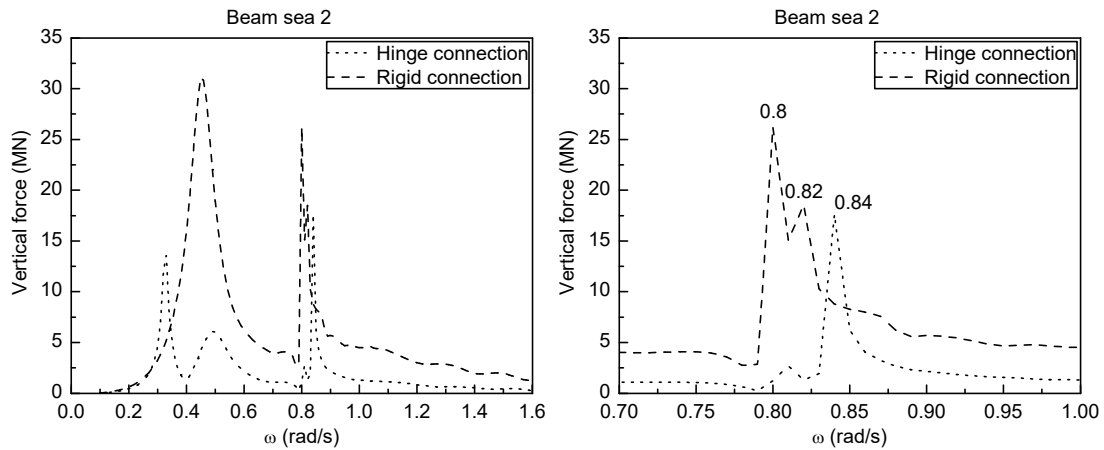
Figure 18. Vertical force in connection in Beam Sea-2
