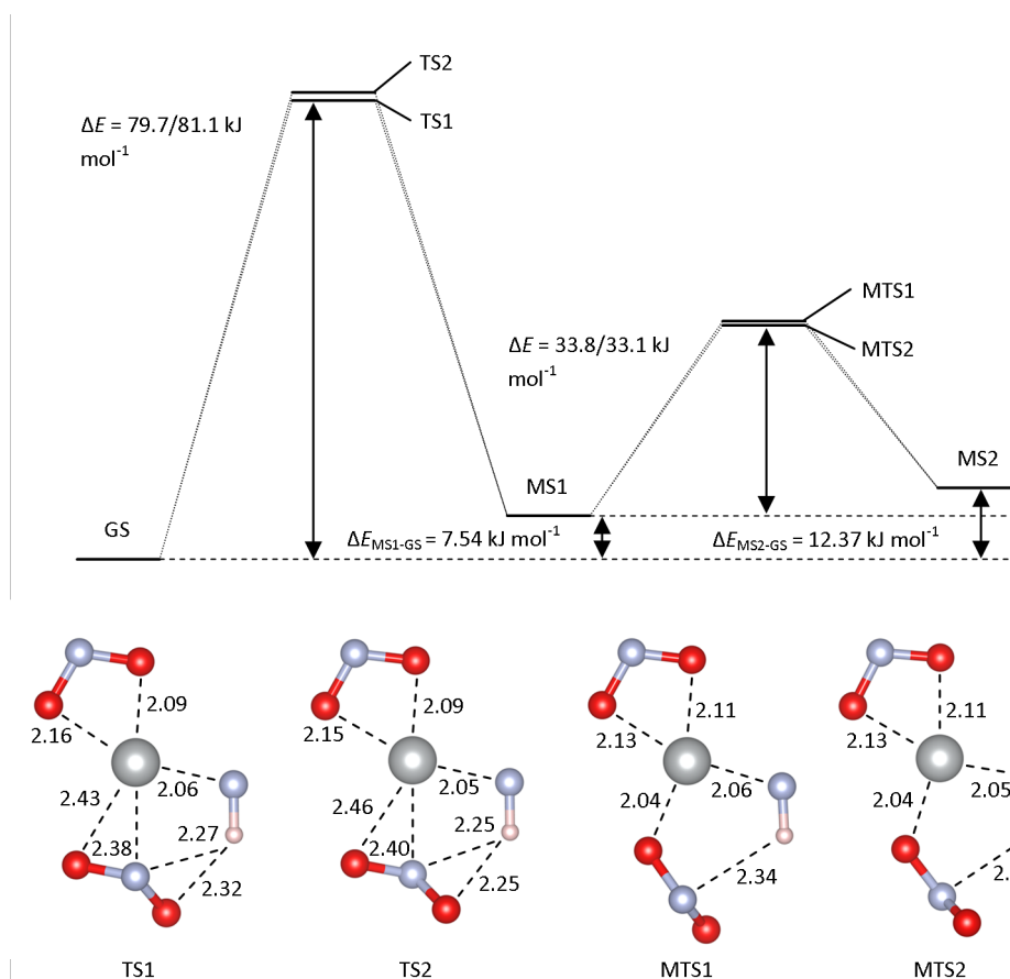
Figure 4 Schematic of the isomerisation pathways in [\text{Ni}(\text{Et}_4\text{dien})(\eta^2\text{-O,ON})(\eta^1\text{-NO}_2)] , modelled using the M06 functional and the LANL2DZ/6-311++G(d,p) basis set, and with water as a continuum. The energy profile illustrates the relative energies of the GS, MS1 and MS2 isomers, and the transition states connecting them, while the four models show the optimised geometries of the four transition states.
