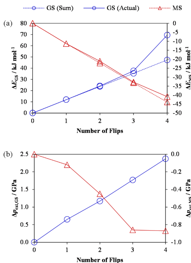
Figure 2 Effect of the GS->MS1 (blue line) and reverse MS1->GS (red line) isomerisation on the energy of (a) and external pressure on ( p_{\text{ext}} ), (b) the GS/MS1 crystal structures. In plot (a), the sum of the energy changes which occur when 1-4 ligands are isomerised in isolation (dashed lines) is compared against the energy change on flipping the same number of ligands in tandem. The energies and stresses are computed from single-point PBEsol+ U calculations performed on the PBEsol-optimised structures. These calculations suggest that the linear increase in the stress on the unit cell with conversion during the GS→MS1 transition makes the final isomerisation energetically more difficult, in the absence of lattice relaxation.
