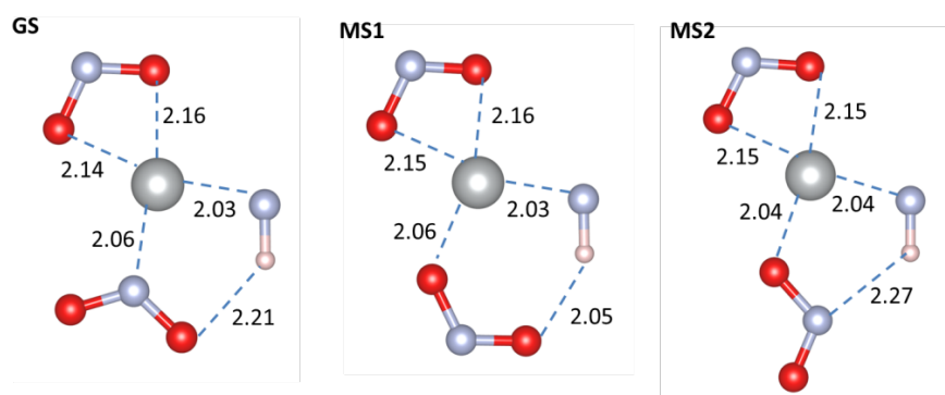
Figure 3 Optimised geometries of the GS, MS1 and MS2 complexes with the M06 functional and the LANL2DZ/6-311++G(d,p) basis set, with water as a dielectric continuum.
