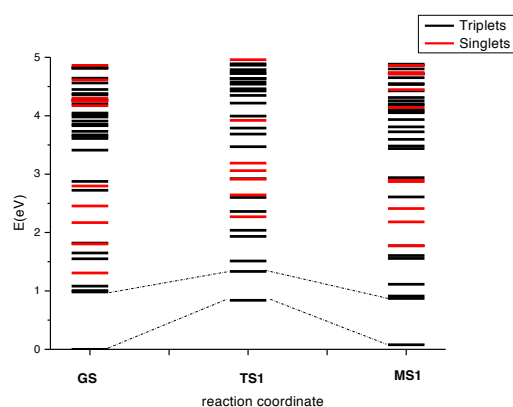
Figure 7 Energy profiles for the GS->MS1 transition in the ground and photoexcited states. Triplet and singlet states are indicated by black and red lines, respectively. The excited states were computed at the TD-DFT/M06/LANL2DZ/6-311++G(d,p) level of theory with water as a continuum.
