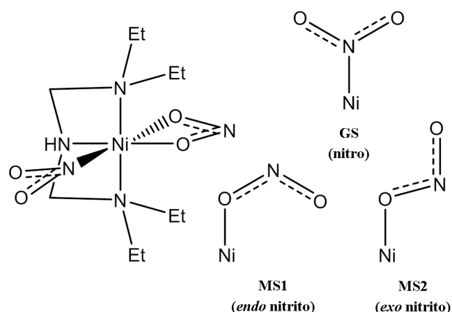
Figure 1 Schematic structure of the [\text{Ni}(\text{Et}_4\text{dien})(\eta^2\text{-O,ON})(\eta^1\text{-NO}_2)] system. The four skeletal drawings show the structure of the molecule (left) and the three different binding modes of the isomerisable \text{NO}_2 group (right), viz. the ground-state (GS) nitro and metastable endo and exo nitrito forms (MS1/MS2, respectively).
