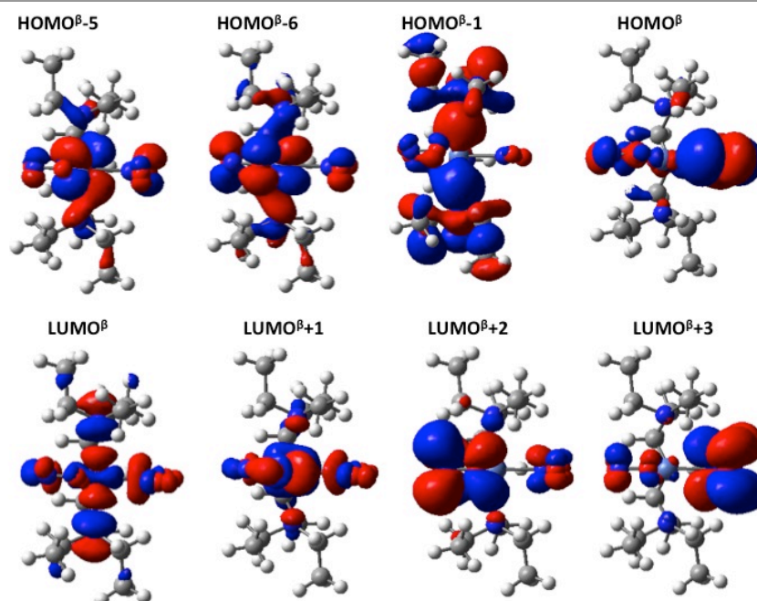
Figure 6 Schematic of the molecular orbitals involved in the most important electronic transitions in the GS isomer, computed with the M06 functional and the LANL2DZ/6-311++G(d,p) basis set with water as a continuum. The labelling convention is based on the beta spin channel (that which does not contain the two unpaired electrons), in which the most important calculated electronic transitions take place.
