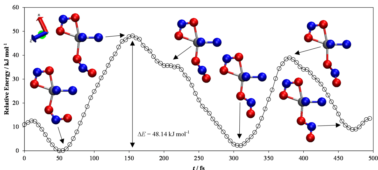
Figure 5 Energy profile for the endo -to- exo transition in [\text{Ni}(\text{Et}_4\text{dien})(\eta^2\text{-O,ON})(\eta^1\text{-NO}_2)] , obtained from constrained ab initio molecular-dynamics simulations. The energies are expressed relative to the lowest-energy point on the curve. Snapshots of the geometry of the complex at various local maxima and minima on the profile are shown, with the atoms colour coded as follows: N - blue, O - red, Ni - silver. The largest energy barrier involved in the switching is 48.14 \text{ kJ mol}^{-1} , and corresponds to a clockwise rotation of the \text{NO}_2 group by approximately 45^\circ from the endo position. The snapshots were created with the VMD software. 44
