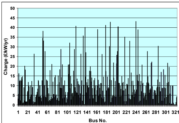
Fig. 3. Long-run incremental charges for the test system
