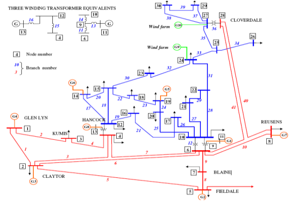
Fig.2. IEEE 30 bus test system [25]
