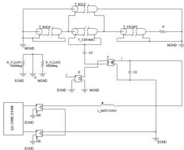
Fig.12 Simulation circuit for switching scheme evaluation.
