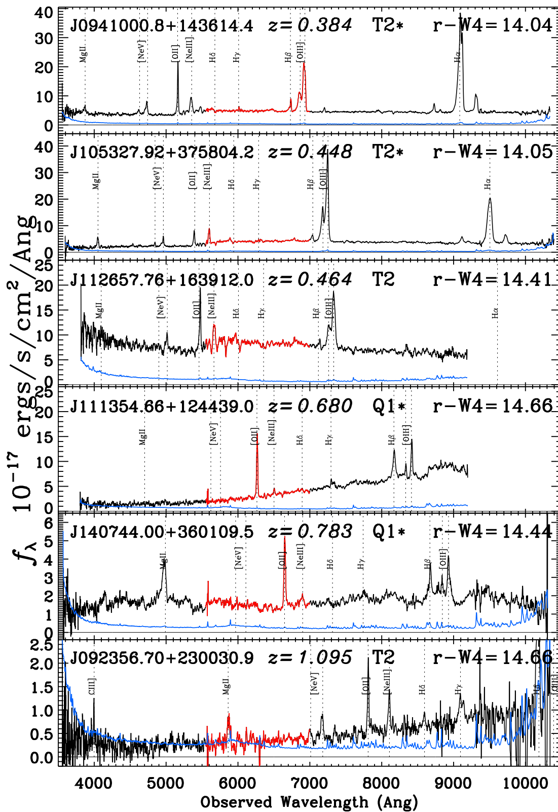
Figure 12. Same as for Fig 9, except showing examples of extremely red quasars that display signatures of an ongoing, or post, star-bursting phase. In particular we identify the Balmer edge in J105327.92+375804.2 and J112657.76+163912.0.
