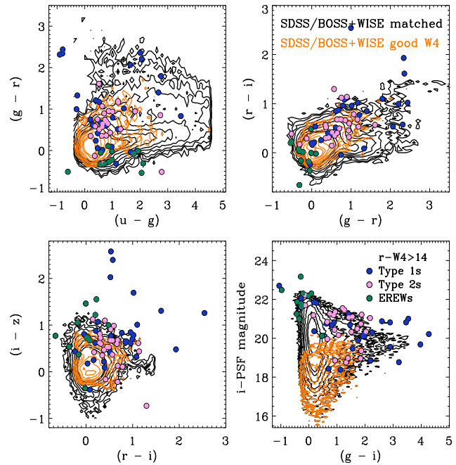
Figure 18. The optical colour-colour properties of SDSS/BOSS+WISE matched sample and the extremely red quasars: ( top left ): (u - g) vs. (g - r) ; ( top right ): (g - r) vs. (r - i) ; ( bottom left ): (r - i) vs. (i - z) ; ( bottom right ): (g - i) vs. i -band PSF magnitude. The distribution of all the SDSS/BOSS quasars with a good match in any WISE band is given by the black contours, while those objects with good W4 -matches, and their colour distributions are given by the solid orange contours. We also show the location in colour-colour space of the three broad groups of our extremely red quasars – Type 1s (dark blue circles), Type 2s (purple) and EREW objects (dark green). The EREWs occupy a particular place in gri -colour-colour space, being very blue in (g - i) colour.
