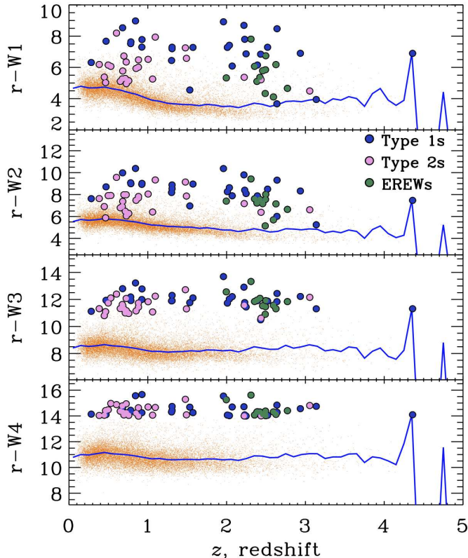
Figure 17. The optical-midinfrared colour for our W4 -matched sample (orange points), with r - W1 , r - W2 , r - W3 and r - W4 shown from top to bottom. The mean colour of the W4 -matched sample is given by the solid blue line. As the optical-MIR wavelength arm extends from W1 ( 3.4\mu\text{m} ) to W4 ( 22\mu\text{m} ) the selected population moves further away from the mean W4 -matched sample. All optical magnitudes are AB, all WISE magnitudes are Vega.
