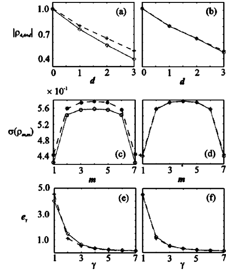
FIG. 2. Comparisons of the numerical ( \circ ) and exact ( * ) calculations with U/2J=2 for spatial correlations |\rho_{4,4+d}| with the central site m=4 obtained for (a) \chi=3 and (b) \chi=5 , the standard deviation of the site occupation \sigma(\rho_{m,m}) obtained for (c) \chi=3 and (d) \chi=5 , and the spectrum e_\gamma of the one-particle density matrix obtained for (e) \chi=3 and (f) \chi=5 . The dashed and dotted curves shown are to guide the eye.
