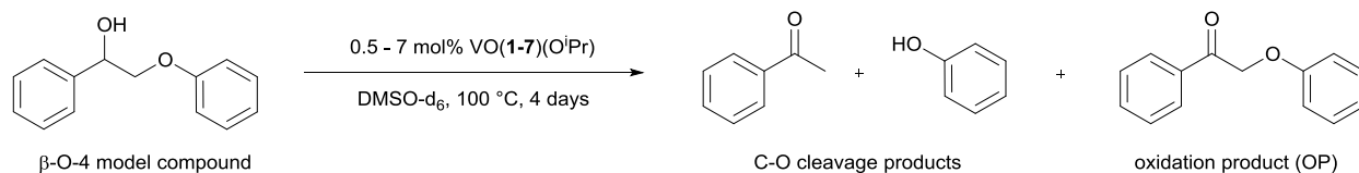
Figure 5: Degradation of \beta -O-4 lignin model compound 2-phenoxy-1-phenylethanol to C-O cleavage products acetophenone and phenol, and benzylic oxidation product (OP) 2-phenoxy-1-phenylethanol.
