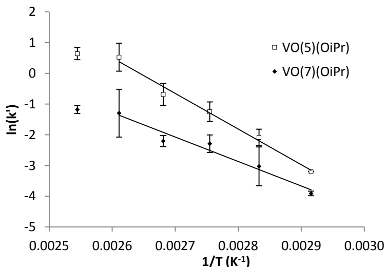
Figure 8: Arrhenius plots for the degradation of 2-phenoxy-1-phenylethanol by VO(5,7)(O i Pr).
