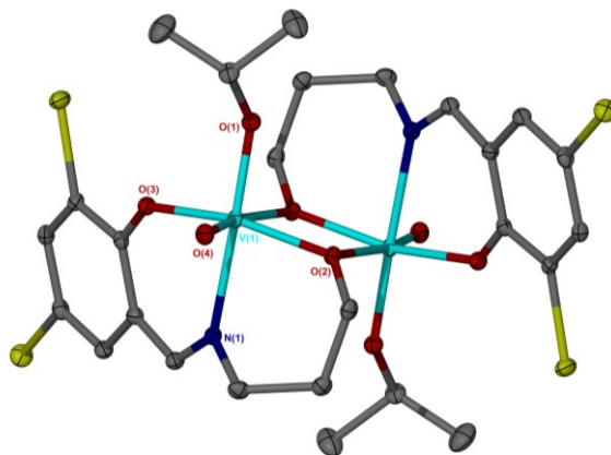
Figure 4: Solid state structure of VO(2)(O i Pr) ellipsoids are shown at the 30% probability level and hydrogen atoms have been removed for clarity.
