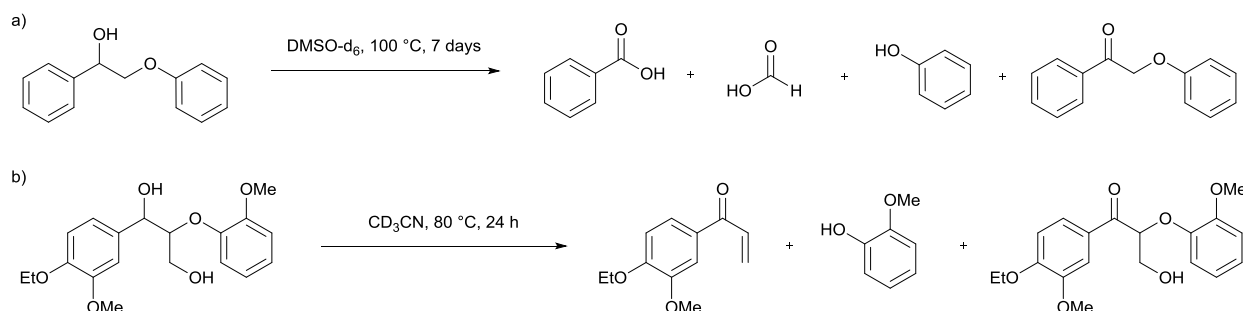
Figure 2: Degradation of \beta -O-4 model lignin compounds by vanadium catalysts a) C-C cleavage and benzylic oxidation, Hanson [17]; b) C-O cleavage and benzylic oxidation, Toste [18]
