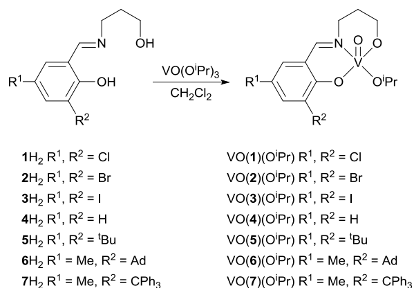
Figure 3: Synthesis of vanadium Schiff-base catalysts
