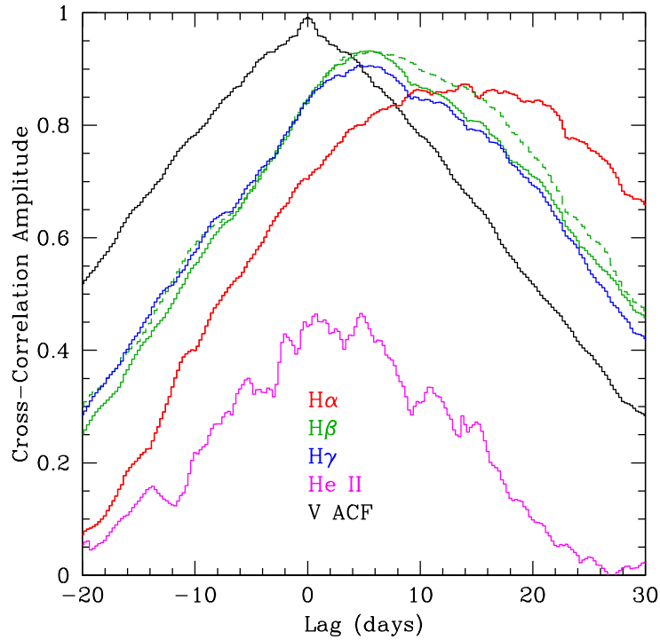
FIG. 3.— Cross correlation functions of H\alpha , H\beta (solid line is the blue side data, dashed line is from the red side), H\gamma and He II against the V-band light curve. Also shown is the autocorrelation function of the V-band continuum.
