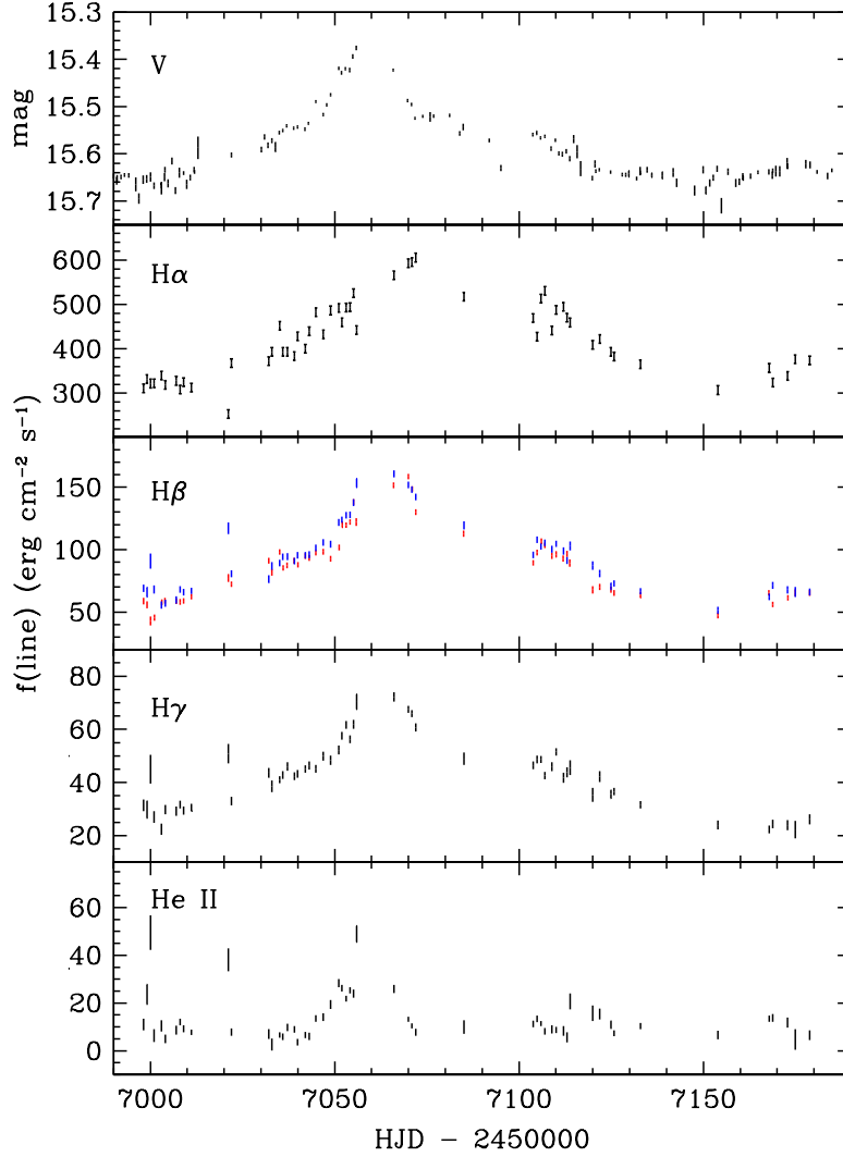
FIG. 1.— Arp 151 light curves for the V -band and the emission lines H\alpha , H\beta , H\gamma , and He II as determined from the FLOYDS spectra. The red and blue points show the H\beta light curve determined from the 1st and 2nd order FLOYDS spectra, respectively, as this emission line is visible in both simultaneously. The normalized excess rms scatter of the [OIII] light curve has been added in quadrature to the photon-counting error bars on each data point to take in account of systematic errors.
