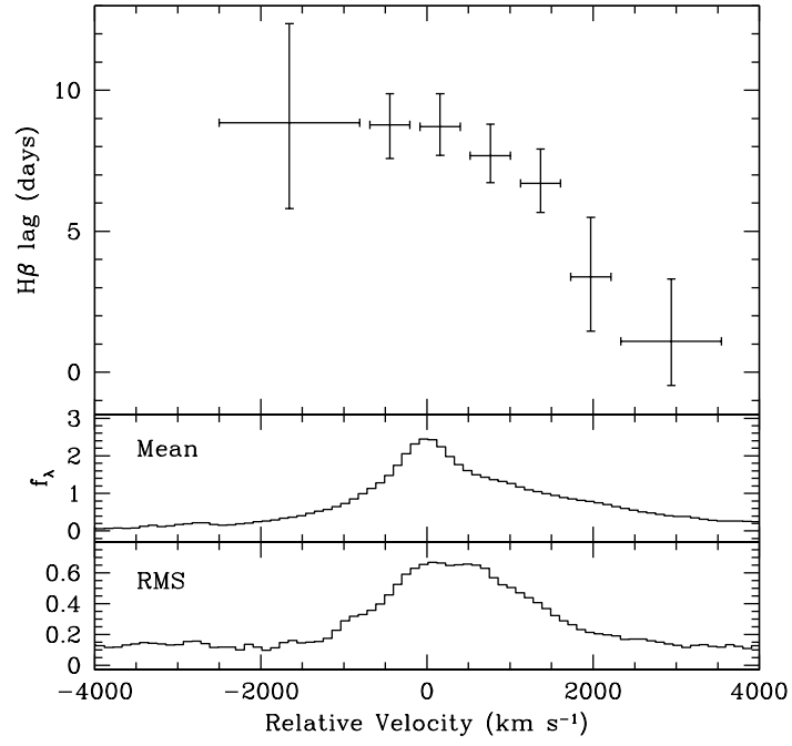
FIG. 4.— Velocity-resolved H\beta lags, as derived from our blue-side FLOYDS data. The upper panel shows the lag (using the \tau_{\text{cen}} measure) for each velocity bin, where the horizontal error bar represents the bin size. The bottom panels show the mean and rms continuum-subtracted spectra.
