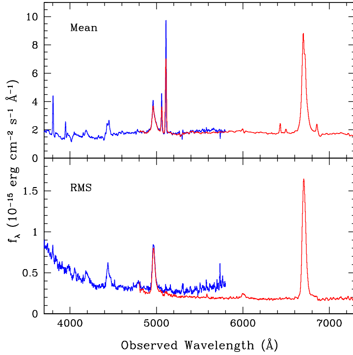
FIG. 2.— Mean and root mean square spectra of Arp 151 from FLOYDS, displaying both the blue and red side spectra. Note that H\beta is in the wavelength overlap region of FLOYDS, and appears in both first and second order. A small flux scaling was applied to the red-side spectrum to match that of the blue side. The upturn in the red side of the blue rms spectrum is due to the lower S/N of the data as the second order throughput of the grating declines.
