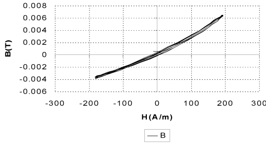
Figure 12: BH Curve derived from FCL operation under nominal load conditions
