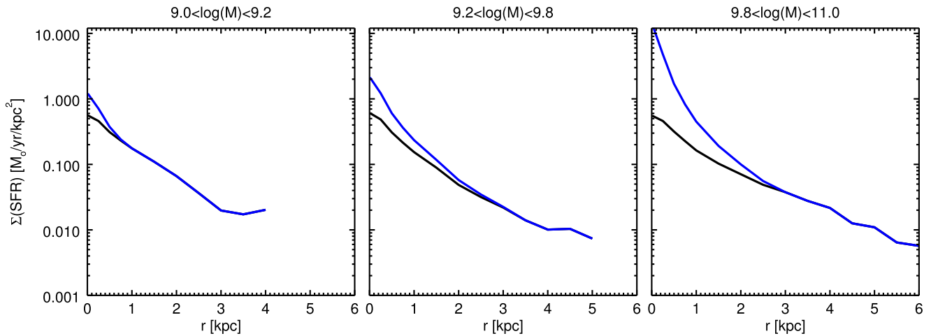
Figure 4. Radial profiles of SFR determined directly from H\alpha emission are shown in black, radial profiles of SFR corrected for dust using radial Balmer decrement profiles are shown in blue. The excess SFR over an exponential toward the center of high mass galaxies suggests we are witnessing the growth of galactic bulges through in situ star formation.
