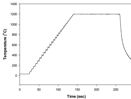
Figure 6: Temperature profile while heating up and cooling down by quenching
