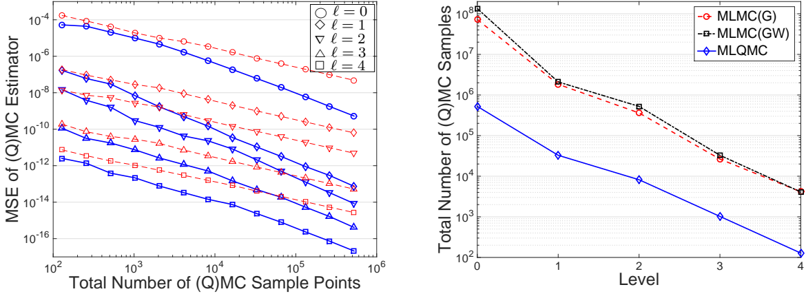
Figure 4: Left: MSE of the QMC/MC estimators for F_\ell - F_{\ell-1} as functions of the total number of sample points, i.e. RN_\ell for QMC (solid blue lines) and N_\ell^{MC} for MC (dashed red lines), for \nu = \sigma^2 = \lambda_C = 1 . Right: Total number of samples on each level to achieve a relative standard error less than \varepsilon = 1.8 \times 10^{-4} for the same example.
