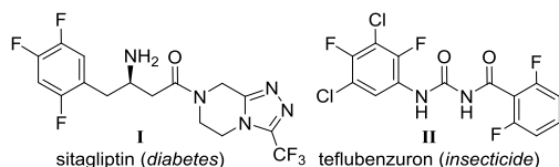
Scheme 1. Examples of commercially important fluorinated molecules.
