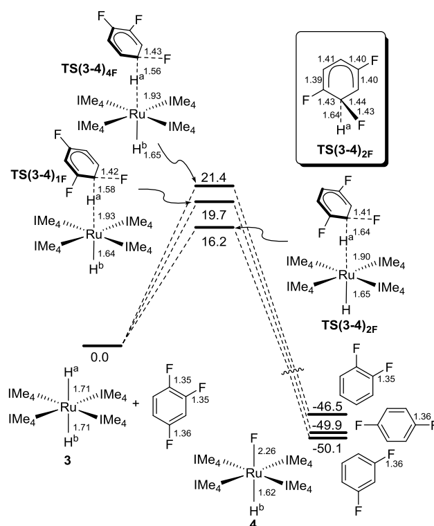
Figure 1. Computed profiles ( \omega B97xD//BP86, free energies in benzene, kcal/mol) for the HDF of 1,2,4-C 6 F 3 H 3 by [Ru(IMe 4 ) 4 H 2 ], 3 . Selected distances are shown in Å and the inset provides additional information for TS(3-4) 2F .
