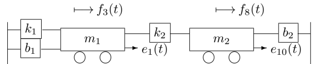
Figure 6. Two-cart system
