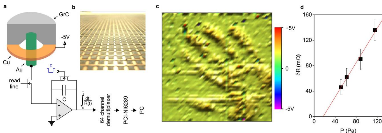
Fig. 4: Fast force field imaging with a 64 × 64 sensor array.
