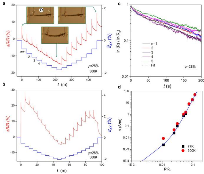
Fig. 1: Transient piezoresistance of composite thin films.
