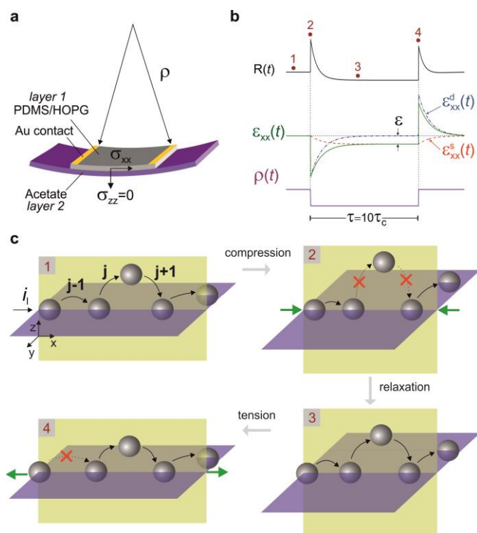
Fig. 2: Perturbative tunnelling model of the linear viscoelastic solid.
