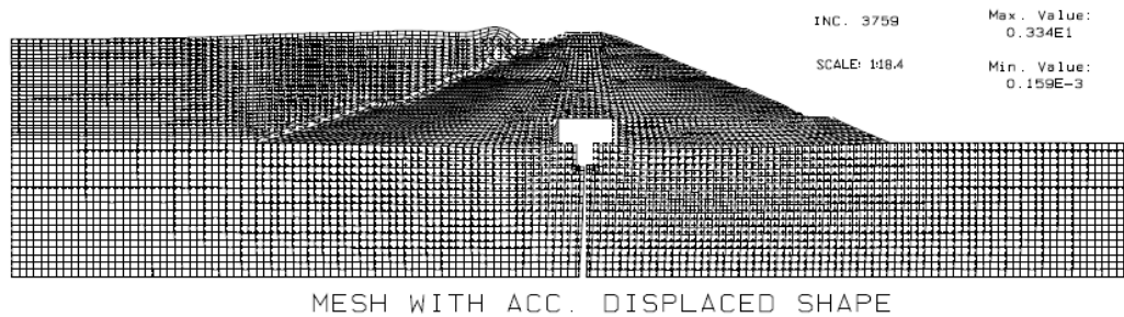
Figure 13: Deformed mesh after the end of EQ5 (Legend values are in meters)
