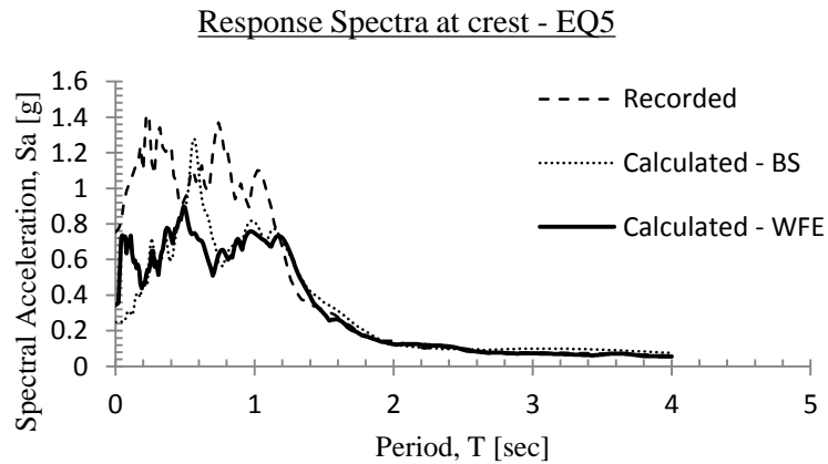
Figure 12: Response spectra of recorded and calculated (both BS & WFE) accelerations at crest for EQ5
