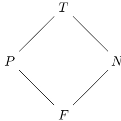
Figure 4: Hasse Diagram for BL.
