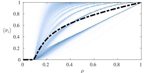
FIG. 1. Micro-structure of percolation in a sample network with 62,586 nodes taken from the gnutella file sharing platform [11]. Each vertical slice of the density plot shows the distribution \varphi(s) of probability to appear in the percolating cluster for given edge occupation probability \rho . The thick dashed line shows the expected size of the percolating cluster S , which is equal to the mean of s under \varphi .
