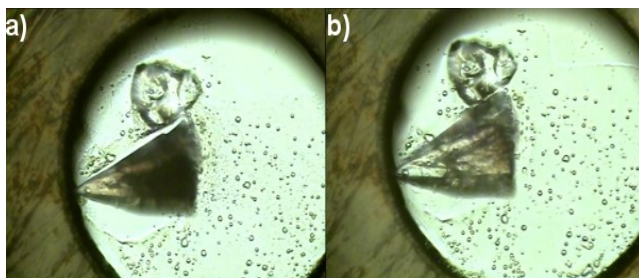
Figure 2. Optical image of \text{Sc}_2\text{BDC}_3 (lower crystal) loaded in Fluorinert FC-77 at (a) 0.40 GPa and (b) 0.10 GPa after decompression. The colourless crystal sitting above \text{Sc}_2\text{BDC}_3 is a chip of ruby, which is used as a pressure calibrant.
