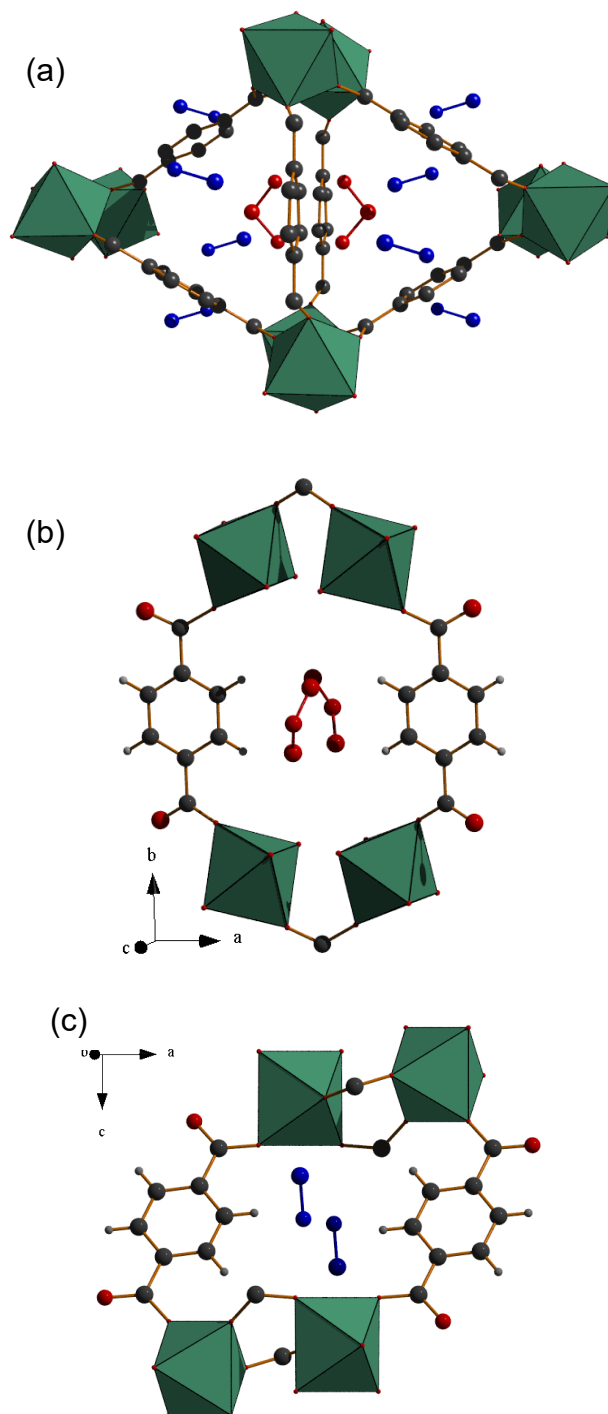
Figure 1. (a) Triangular pores formed in Sc_2BDC_3 viewed along the a -axis. Disordered methanol molecules are represented by solid red (Site 1) and blue (Site 2) coloured molecules. Openings between triangular channels of Sc_2BDC_3 between (b) Group 1 and (c) Group 2 ligands as viewed along the c and b -axes, respectively. Key: C, grey; ScO_6 octahedra, green; O, red; H, light grey.
