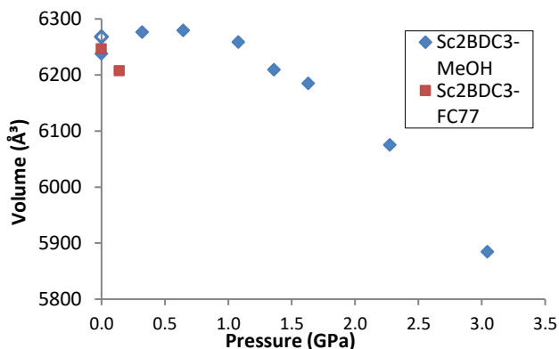
Figure 3a. Unit cell volume of \text{Sc}_2\text{BDC}_3 in methanol and Fluorinert FC-77 as a function of pressure. The open diamond refers to the ambient structure surrounded with MeOH in a capillary.
