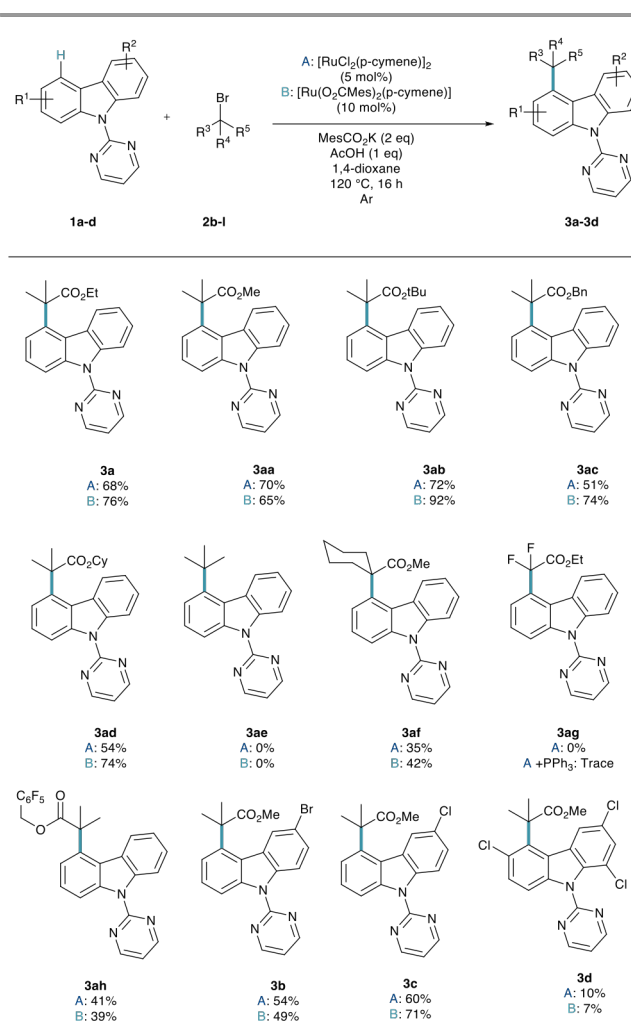
Scheme 2: Ruthenium Catalyzed C4-Selective C-H Alkylation of Carbazole Derivatives
