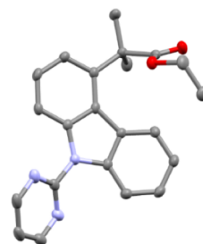
Figure 1: SCXRD Structure of 3a Confirming Regioselectivity of Functionalisation. 19 CCDC 1574475.
