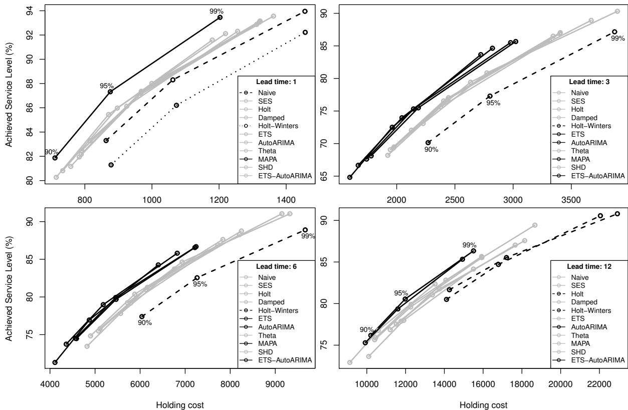
Figure 4: Trade-off curves of holding cost versus achieved service levels for different methods and lead times.
