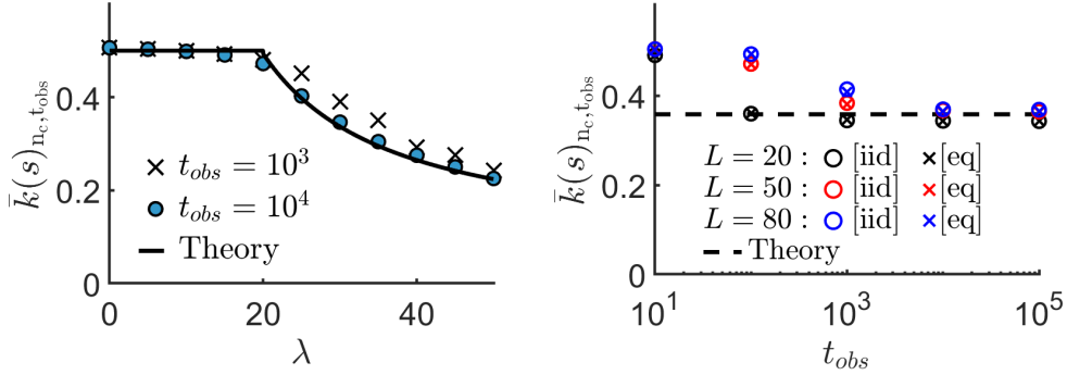
Figure 7: Estimates \bar{k}(\lambda) of the activity \mathcal{K}_L(\lambda) as a function of t_{\text{obs}} for various system sizes L . (a) L = 50 for various \lambda, t_{\text{obs}} . (b) \lambda = 28 for various t_{\text{obs}}, L . The “theory” line is \mathcal{K}_* = \lim_{L \rightarrow \infty} \mathcal{K}_L(\lambda) . We took R = 10 , with n_c = 10^5 for L = 20, 50 and n_c = 10^6 for L = 80 (these n_c are large enough that results depend very weakly on n_c .)
