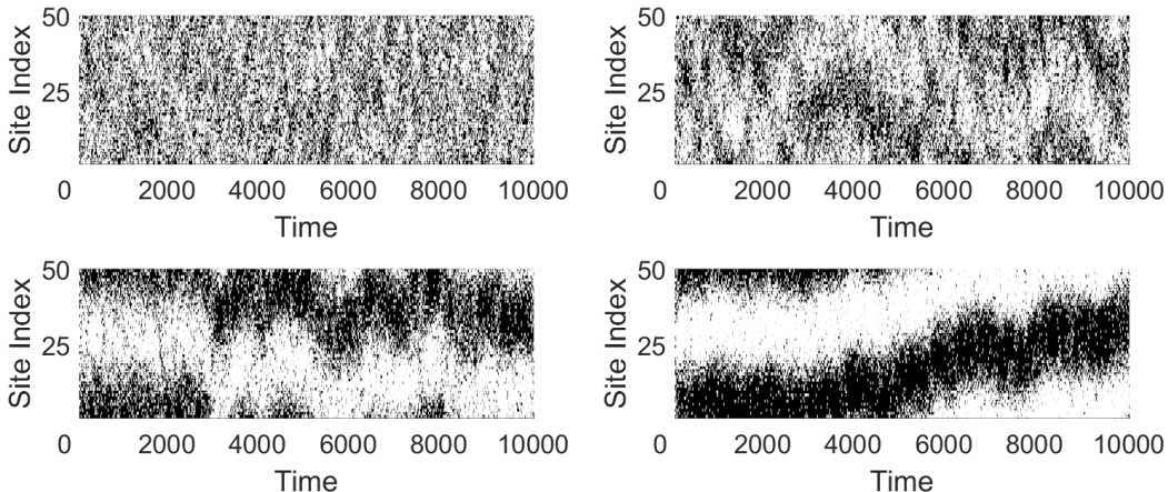
Figure 2: Sample trajectories of SSEP with L = 50 and t_{\text{obs}} = 10^4 . (a) s = 0 , the equilibrium state; (b) s = 0.008 , showing evidence of transient clusters; (c) s = 0.012 , in which a single large cluster has formed; (d) s = 0.020 , with most of the particles in a well-defined single cluster. The corresponding values of \lambda are 0, 20, 30, 50.
