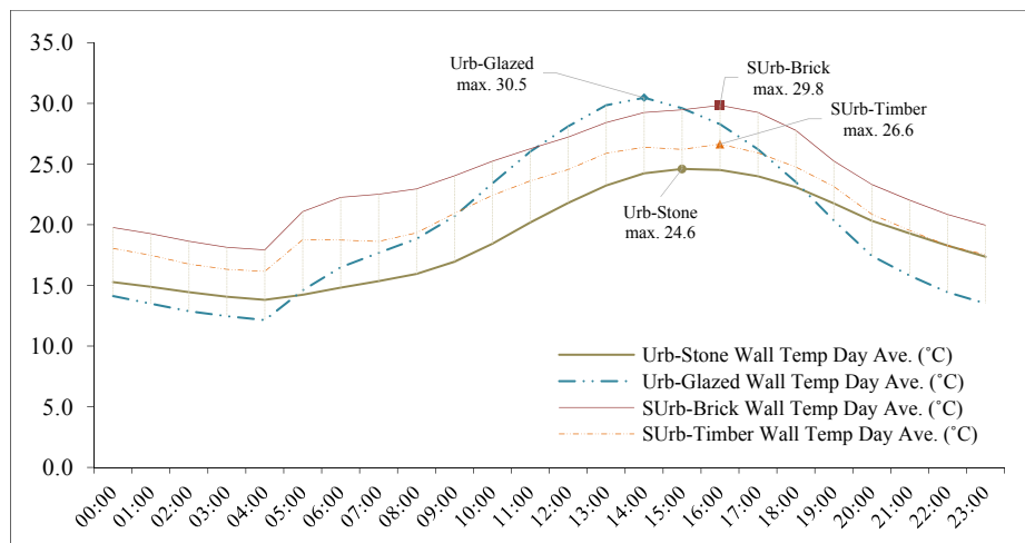
Fig. 10. Summer solstice (21-June) building external wall surface temperatures ( ^{\circ}\text{C} ).
