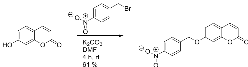
Scheme 1 – Synthesis of NCOU1
