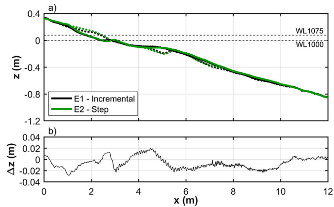
Fig. 5. Comparison of test E1 (incremental water level rise, wave action = 2040 min) and E2 (single step water level rise, wave action = 2150 min). a) profiles; thin dashed lines are the initial profiles developed at WL1000, thick lines are the final profiles at WL1075, b) difference between the final WL1075 profiles of each test.
