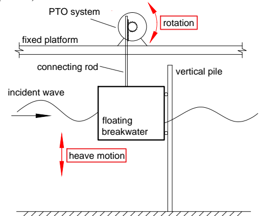
Figure 1: Sketch (side view) of the integrated system.
