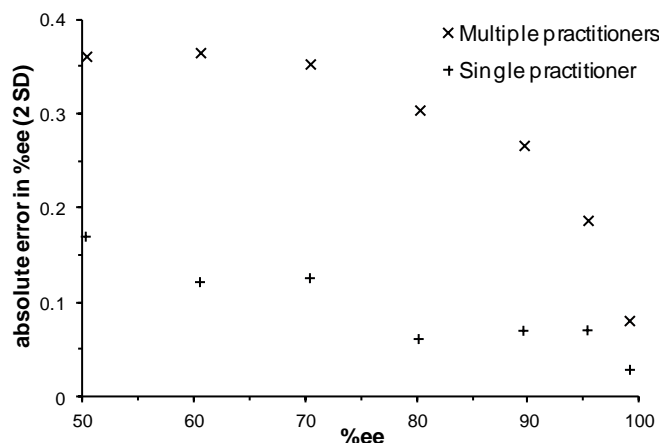
Figure 4. Calculated analytical error in %ee values measured using HPLC analysis. + Each data point obtained from 10 analyses by a single practitioner; x Each data point obtained from 14 analyses by 14 different practitioners.
