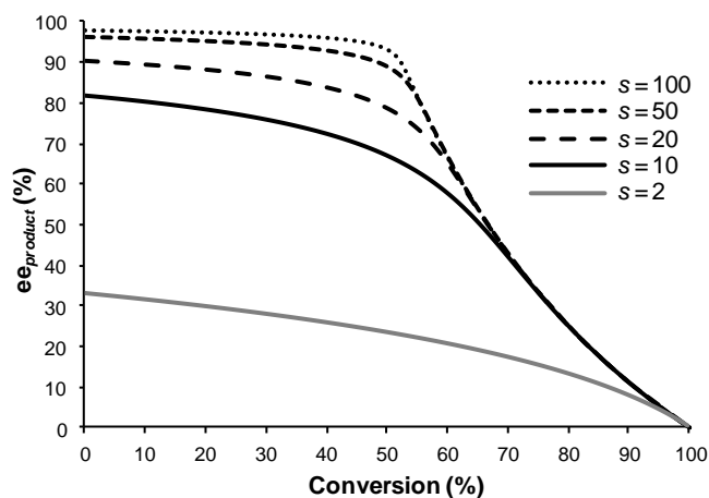
Figure 2. Evolution of %ee of product with reaction conversion.
