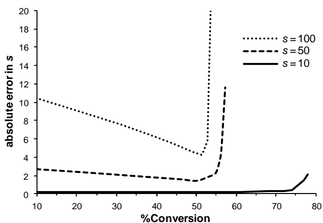
Figure 6. Absolute error in s as a function of reaction conversion.
