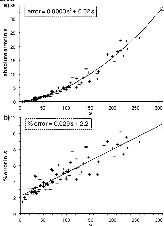
Figure 5. Error in s as a function of s : a) absolute error; b) % error.
